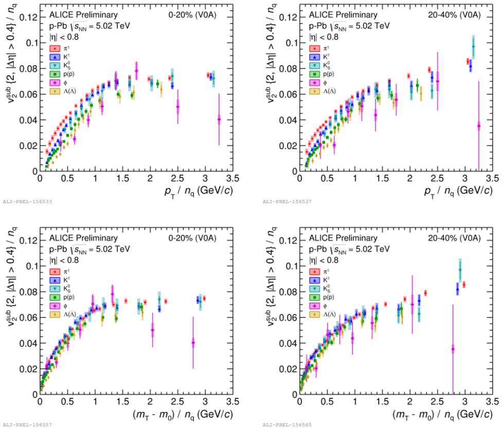
Fig. 2. Test of scaling properties of v_2 coefficients. Upper: both v_2^{\text{sub}} and p_T are scaled by number of constituent quarks n_q (NCQ scaling). Lower: transverse kinetic energy (KE T ) scaling, where rest mass m_0 of individual species is subtracted from m_T .
