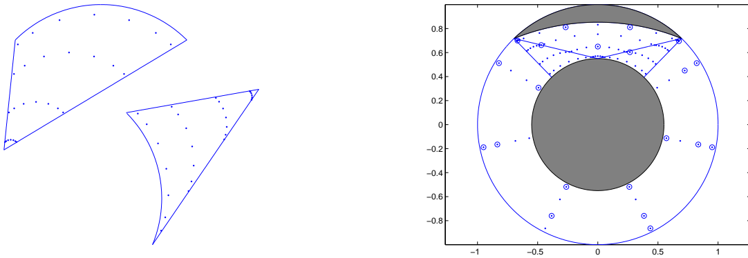
Figure 1: Left: a convex and a concave generalized sector with 28 quadrature nodes ( \cdot ) for polynomial exactness degree n = 5 ; Right: 108 quadrature nodes ( \cdot ) for n = 5 on an obscured and vignetted pupil, and compression into 21 points ( \circ ) by NNLS.
