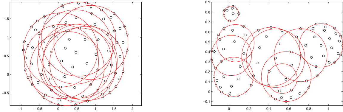
Figure 5: Quadrature nodes on two unions of 10 disks, for degree n = 12 .
