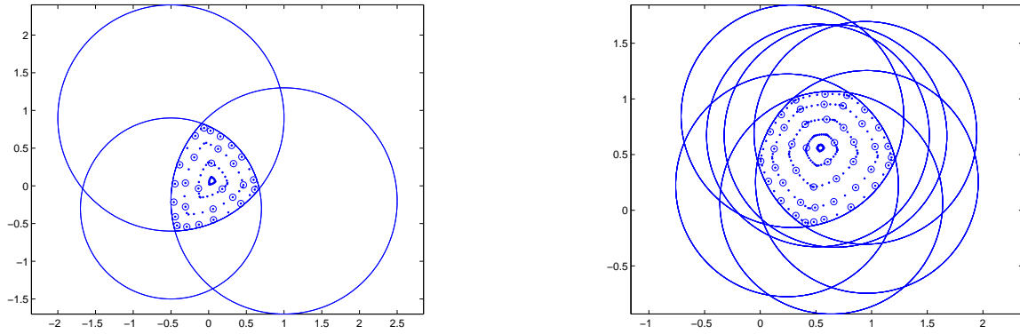
Figure 2: Left: 96 = 32 \times 3 quadrature nodes ( \cdot ) for n = 6 on the intersection of 3 circles and compression into 28 nodes ( \circ ) by NNLS; Right: 250 = 50 \times 5 quadrature nodes for n = 8 on a curvilinear pentagon (intersection of 7 circles with equal radius) and compression into 45 nodes.
