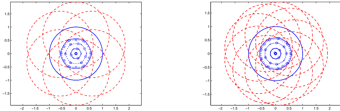
Figure 4: Quadrature nodes for two diaphragms, degree n = 5 ; Left: 6-blade diaphragm, aperture 0.6, blade curvature 0.8, 28 \times 6 = 168 nodes (·) compressed by QR with column pivoting into 21 (○); Right: 9-blade diaphragm, aperture 0.8, blade curvature 0.8, 28 \times 9 = 252 nodes compressed by NNLS into 21.
