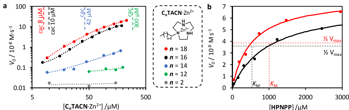
Figure 4. Effect of chain length on catalytic activity. a. Initial speed of HPNPP hydrolysis at increasing C_n\text{TACN}\cdot\text{Zn}^{2+} concentration ( n = 2 to 18, see legend, [\text{HPNPP}] = 500 \mu\text{M} , [\text{HEPES buffer}] = 5 \text{ mM} ), the dotted lines serve as a guide for the eye. b. Initial speed of HPNPP hydrolysis at increasing HPNPP concentration, and fixed C_n\text{TACN}\cdot\text{Zn}^{2+} concentration ( [C_n\text{TACN}\cdot\text{Zn}^{2+}] = 50 \mu\text{M} , [\text{HEPES buffer}] = 50 \text{ mM} ), the solid line are the data fit according to a Michaelis-Menten mechanism. Experiments were performed in aqueous buffer at pH 7, at 40^\circ\text{C} .
