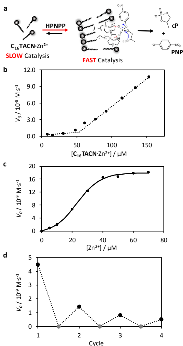
Figure 3. a. Cooperative catalysis induced by neighbouring TACN-Zn 2+ complexes upon assembly. b. Initial speed of HPNPP hydrolysis at increasing C 16 TACN-Zn 2+ concentrations ([ HPNPP ] = 62 μM), the dotted lines are the linear fit to the first three and last three data points. c. Initial speed of HPNPP hydrolysis at a fixed concentration of C 16 TACN and varying Zn 2+ concentrations ([HEPES buffer] = 5 mM, [ C 16 TACN ] = 50 μM, [ HPNPP ] = 500 μM, 40 °C); the solid line represents the sigmoidal fit of the experimental data. d. Initial rates of HPNPP hydrolysis after successive additions of HPNPP (125 μM each addition) in the presence [HEPES buffer] = 5 mM and [ C 16 TACN-Zn 2+ ] = 50 μM at 40 °C. Black data points represent the rate directly after each addition, Grey data points represent the rate after 48 hours just before addition of the new batch of fuel.
