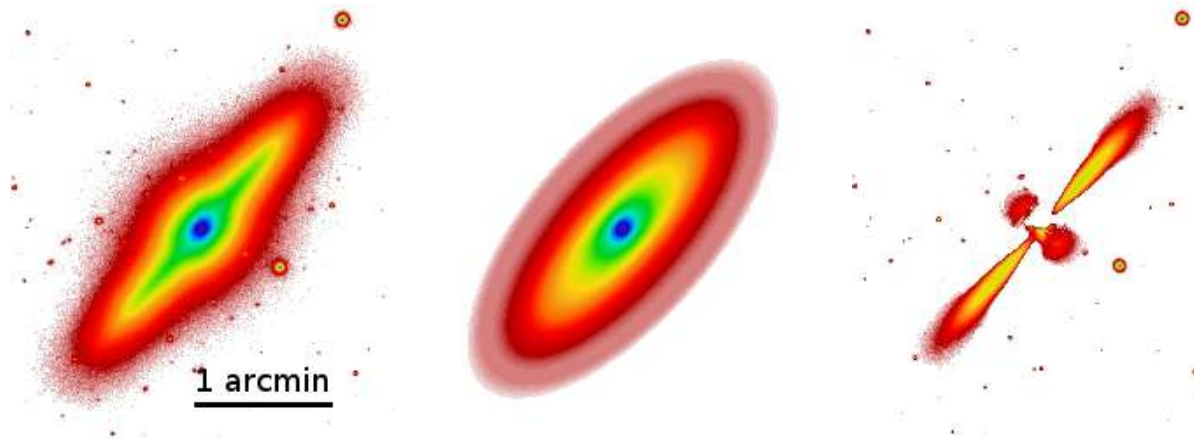
Fig. 10. Isophotal analysis for FCC 170 in the r -band from (Iodice et al. 2019; Fig. 14). From left to right panels: data from the FDS (Iodice et al. 2016), bi-dimensional model and residual image. The latter was obtained subtracting the model from the data and clearly shows the thin disk flaring.
