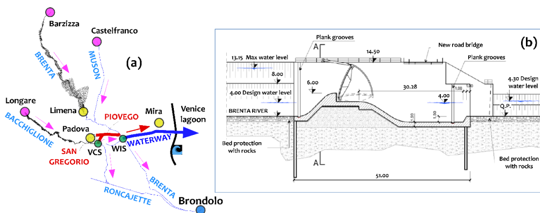
Figure 3. (a) Domain of the study and the computational mesh used to model flood propagation in the Brenta–Bacchiglione river network. Violet points denote the inflow boundary conditions; green points are the hydraulic facilities (the Voltabarozzo control structure, VCS, and the waterway intake structure, WIS); the blue point locates the mouth of the Brenta in the Adriatic Sea at Brondolo. (b) Details of the waterway intake structure (WIS).
