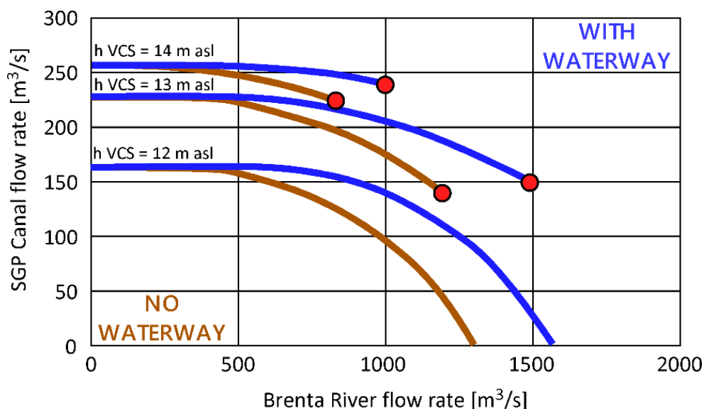
Figure 4. Maximum flow rates that can be conveyed through the SGP Canal into the Brenta River (i.e., gates of the Scaricatore facility were completely open) as a function of the flow rates in the Brenta River. Brown lines represent the current condition, blue lines represent the effect of using the waterway of Padova–Venice as a diversion canal. Different set of lines refer to different water level upstream of the VCS; red circles denote the maximum discharge through the SGP Canal for which the levees are not overtopped.
