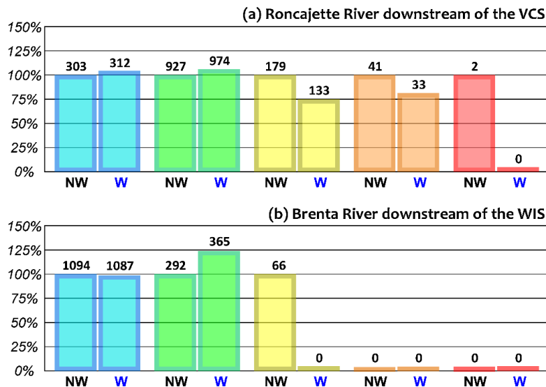
Figure 7. Effect of the waterway as a diversion canal on hydraulic risk in the Brenta–Bacchiglione river network. The number of hours (bold numbers) spent in each of the risk classes defined in Section 2.1.1, using (W) and without using (NW) the Waterway as diversion canal, for the Roncayette River (a) and for the Brenta River downstream of the WIS (b). Histogram bars are normalized with respect to the case of no waterway use.
