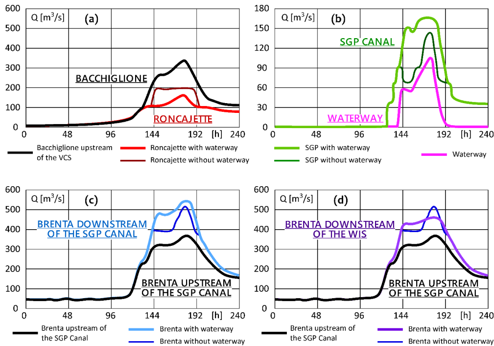
Figure 6. Simulation of the 01–10 November 2011 flood event. Comparisons between flow rates computed, without (current conditions, dark colors, thin lines) and with (light colors, thick lines), the use of the waterway as a diversion canal. Black lines represent the flow rates upstream of Padova. The waterway allows—(a) reducing the flow rates in the Roncayette River, (b) increasing the flow rates of the Bacchiglione River that the SGP Canal could divert to the Brenta River (green lines), (c) increasing the flow rates of the Brenta River between the confluence of Piovego–Brenta and the WIS (blue lines) without increasing the water levels, and (d) flattening the flood hydrograph of the Brenta River downstream of the WIS.
