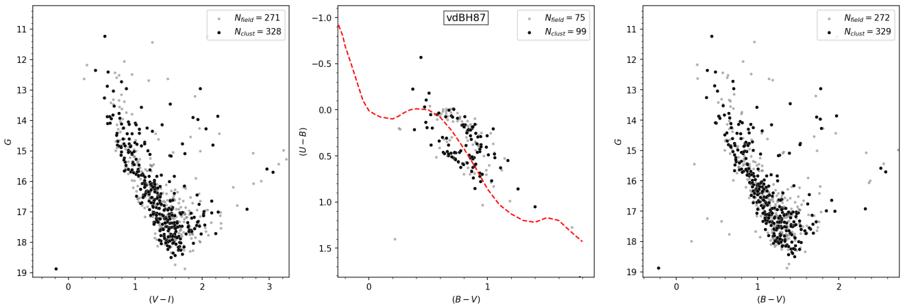
Fig. A.9. Same as Fig. 4 for vdBH 87.
