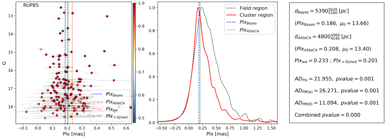
Fig. A.8. Same as Fig. 7 for RUP 85.
