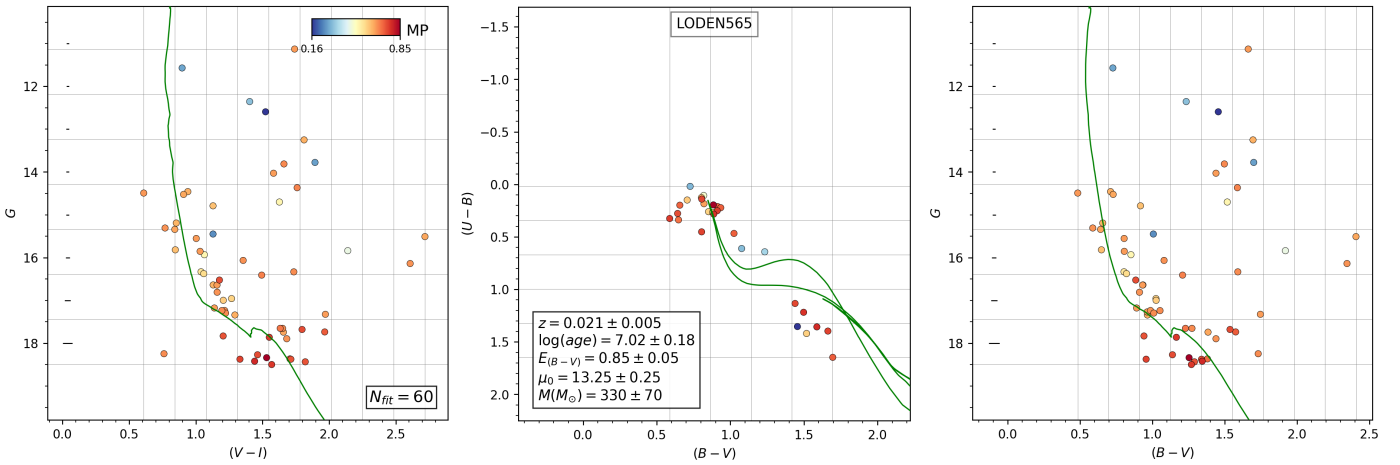
Fig. A.47. Same as Fig. 6 for Loden 565.
