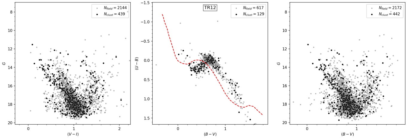
Fig. A.17. Same as Fig. 4 for TR 12.
