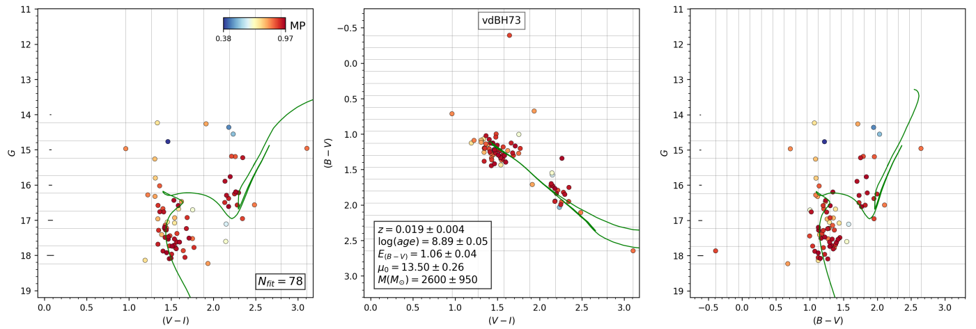
Fig. A.3. Same as Fig. 6 for vdBH 73 with the (B - V) vs. (V - I) diagram instead of the (B - V) vs. (U - B) diagram.
