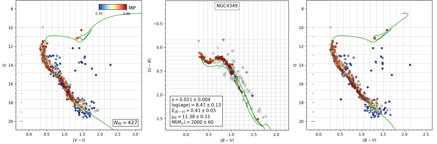
Fig. 10. Same as Fig. 6 for NGC 4349.
