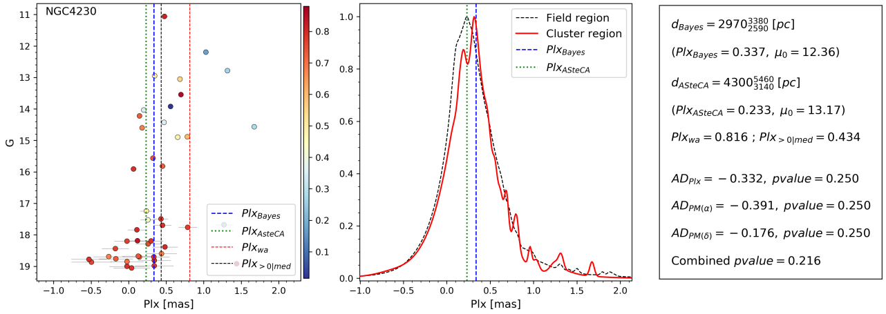
Fig. A.52. Same as Fig. 7 for NGC 4230.
