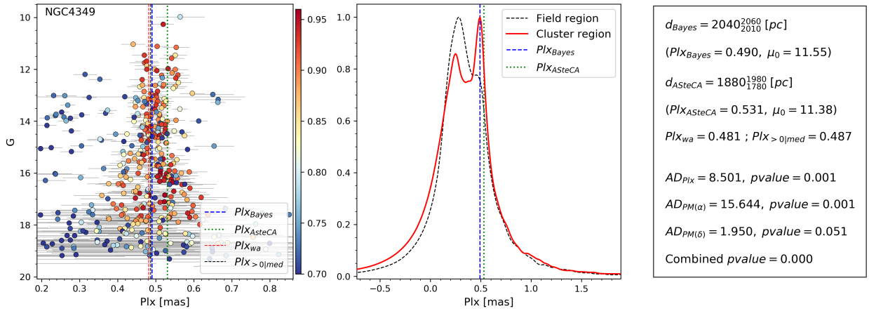
Fig. 11. Same as Fig. 7 for NGC 4349.
