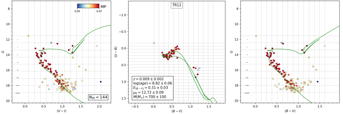
Fig. A.19. Same as Fig. 6 for TR 12.
