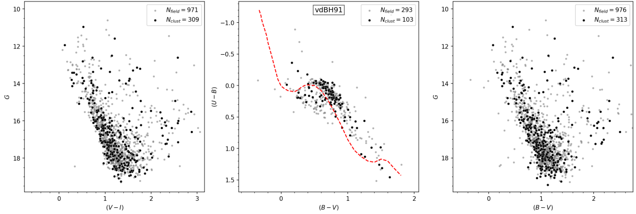
Fig. A.21. Same as Fig. 4 for vdBH 91.
