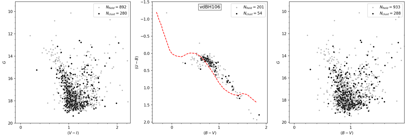
Fig. A.29. Same as Fig. 4 for vdBH 106.
