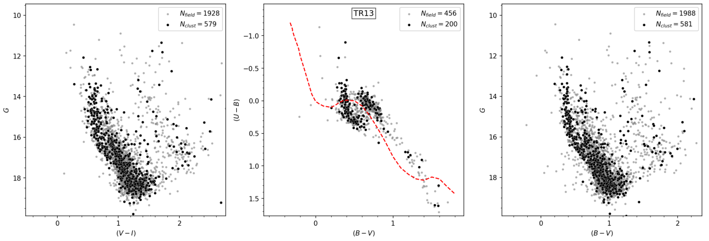
Fig. A.25. Same as Fig. 4 for TR 13.
