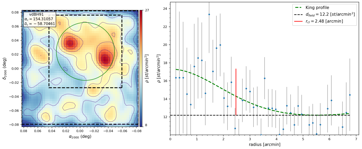
Fig. A.22. Same as Fig. 5 for vdBH 91.
