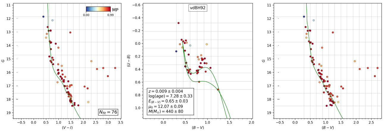
Fig. A.15. Same as Fig. 6 for vdBH 92.
