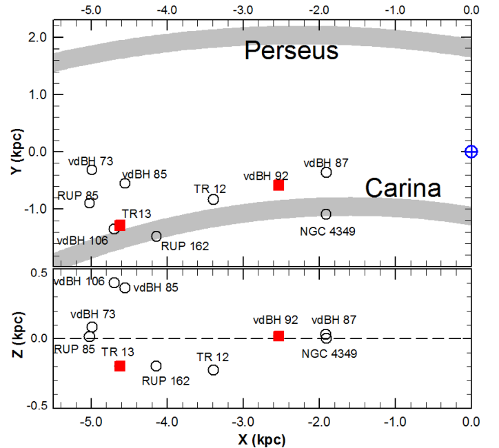
Fig. 17. X – Y (upper panel) and X – Z (lower panel) projection of the true and probable clusters in our sample (open circles). The red squares enclose the youngest clusters in our list (see Table 4). The thick gray lines in the upper panel show the trace of the Perseus and Carina arms according to Vallée (2005). The position of the Sun is shown by a blue crossed circle. The dashed line in the lower panel depicts the Galactic equator.
