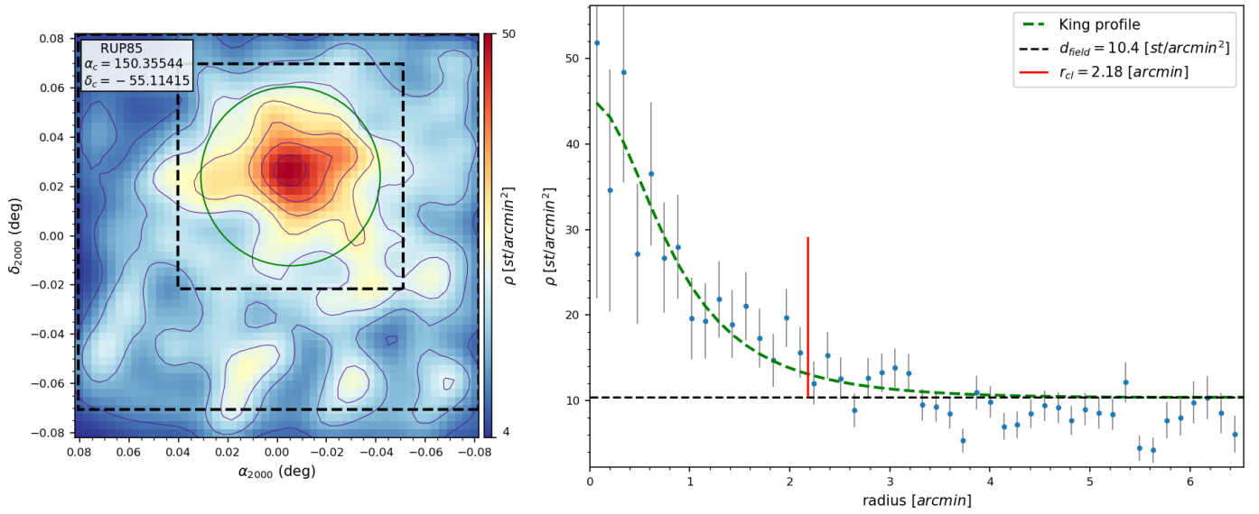
Fig. A.6. Same as Fig. 5 for RUP 85.
