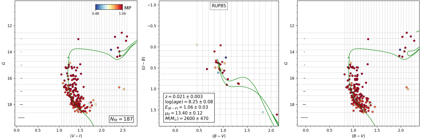
Fig. A.7. Same as Fig. 6 for RUP 85.
