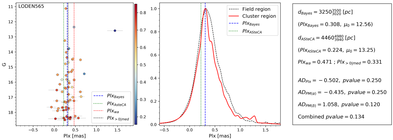
Fig. A.48. Same as Fig. 7 for Loden 565.
