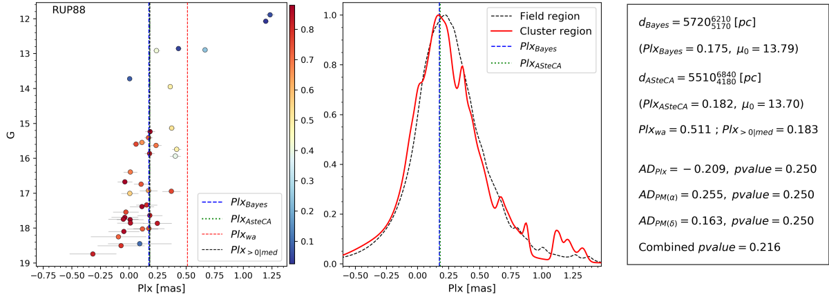
Fig. A.36. Same as Fig. 7 for RUP 88.
