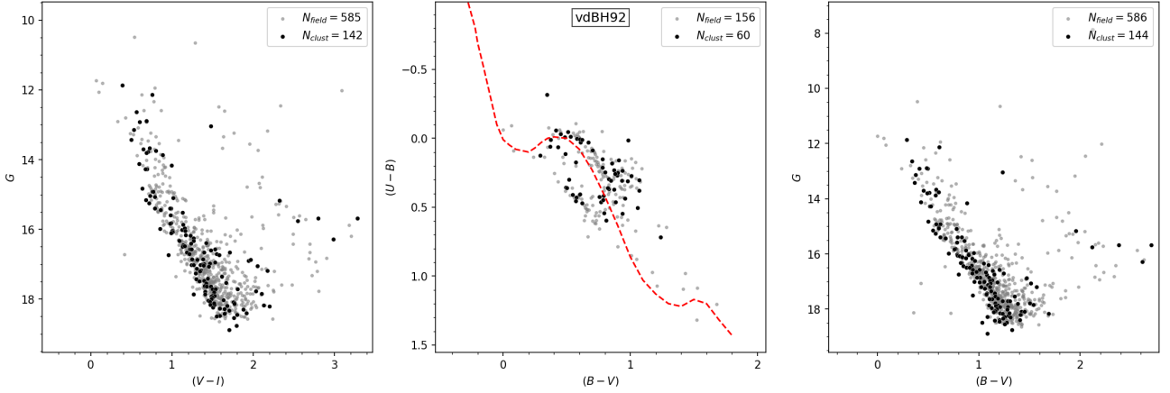
Fig. A.13. Same as Fig. 4 for vdBH 92.
