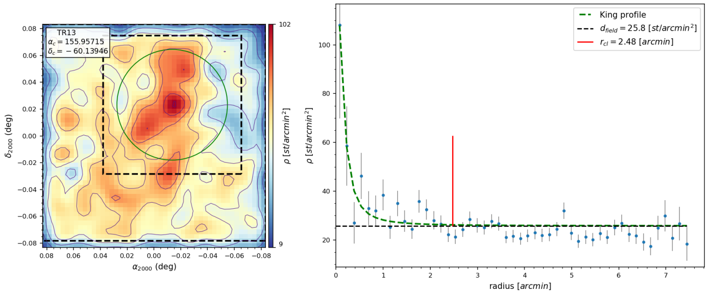
Fig. A.26. Same as Fig. 5 for TR 13.
