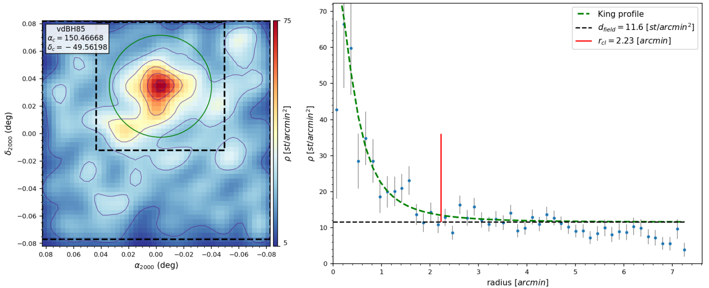
Fig. 5. From left to right, we present in the first panel a contour plot showing the position of the overdensity associated with vdBH 85. The green inner circle shows the cluster size, and the two black dashed-line squares enclose the region that ASteCA used to estimate the field stellar properties. The lower density values at the frame borders are an artifact of the kernel density estimate method that we employed to generate the density maps. Equatorial coordinates in decimal format are indicated. The color bar denotes the star number per square arcminute (linear scale). These values are slightly different from those in the panel to the right because they are obtained with a different method (nearest neighbors). The second panel shows the RDP as blue dots with standard deviations as vertical black lines. The King profile is shown as a dashed green line. The horizontal black line is the mean field stellar density. The vertical red line is the adopted cluster radius.
