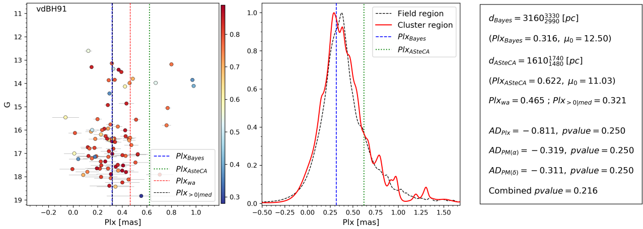
Fig. A.24. Same as Fig. 7 for vdBH 91.
