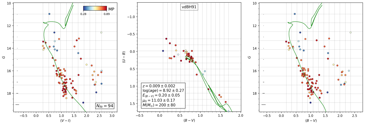
Fig. A.23. Same as Fig. 6 for vdBH 91.
