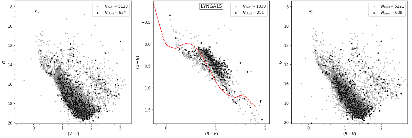
Fig. A.41. Same as Fig. 4 for Lynga 15.
