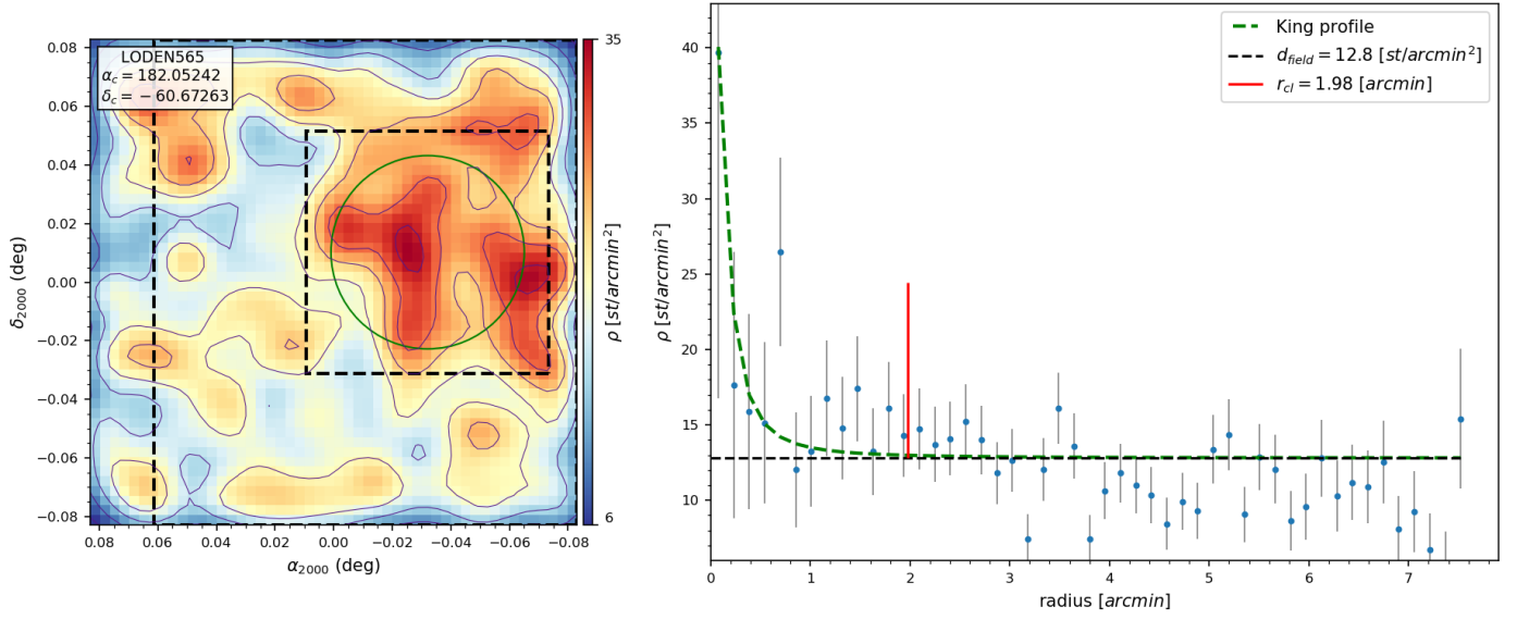
Fig. A.46. Same as Fig. 5 for Loden 565.
