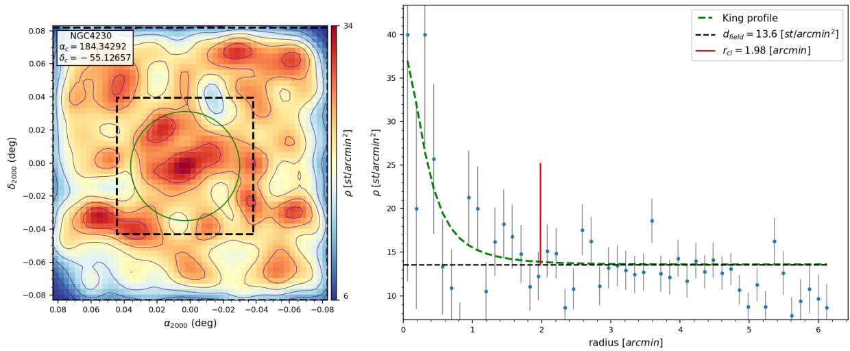
Fig. A.50. Same as Fig. 5 for NGC 4230.
