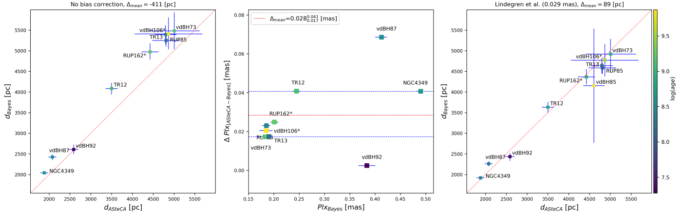
Fig. 16. Left: ASteCA (photometric) vs. Bayesian (parallax) distances for the clusters listed in Table 4 that are confirmed to be real clusters. No bias correction was applied to the parallax data. The color bar at the right indicates \log(\text{age}) values. Center: offset (ASteCA – Bayes) for distances expressed as parallax in milliarcseconds. Right: same as left plot, with bias corrections from Lindegren et al. (+0.029 mas). The cluster vdBH85 is included here; its distance value is estimated from the list of individual distances reported by Bailer-Jones et al. (2018).
