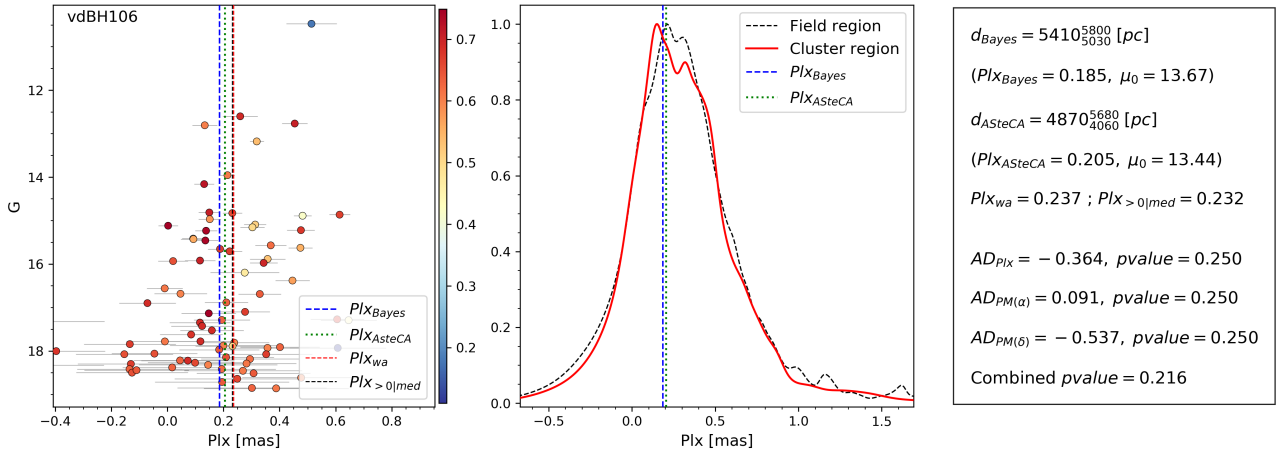
Fig. A.32. Same as Fig. 7 for vdBH 106.
