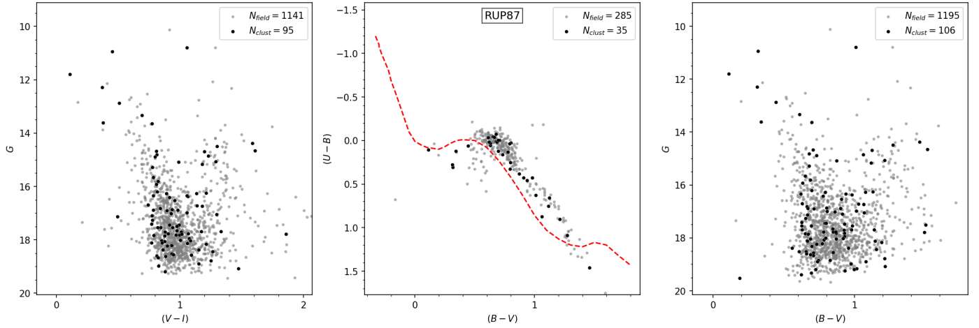
Fig. 12. Same as Fig. 4 for RUP 87.
