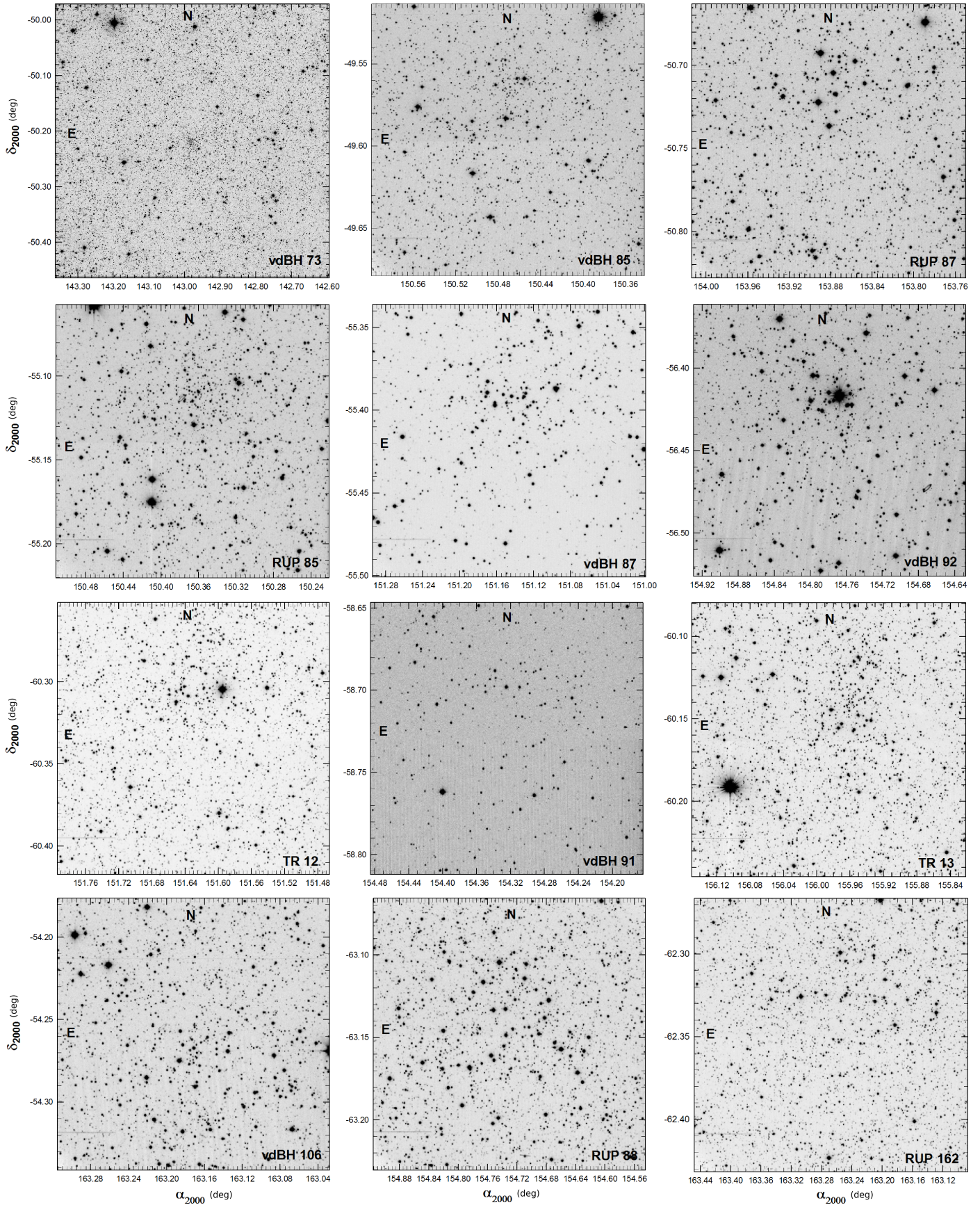
Fig. 3. V images (charts) of the observed clusters (names inserted) ordered from top to bottom and from left to right by increasing longitude. Decimal \alpha and \delta coordinates for the 2000 equinox are indicated. North and east are also shown.
