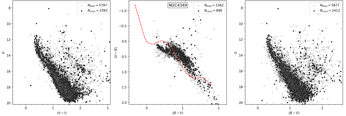
Fig. 8. Same as Fig. 4 for NGC 4349.
