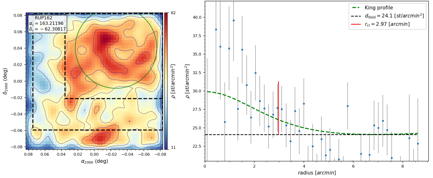
Fig. A.38. Same as Fig. 5 for RUP 162.
