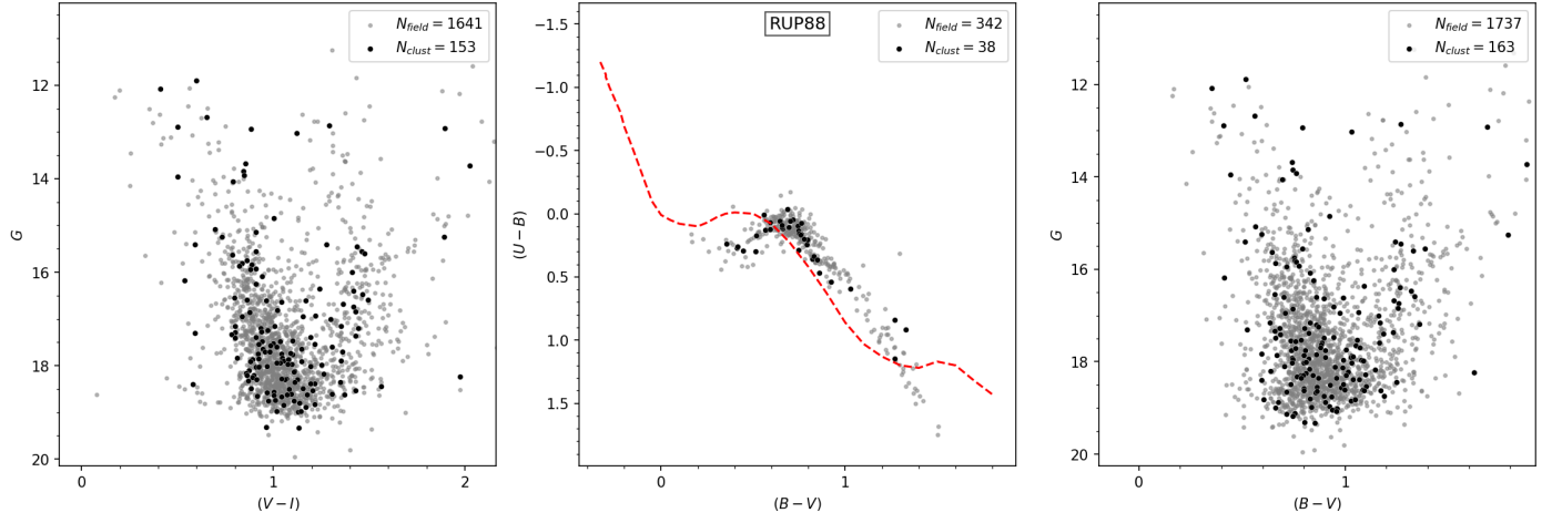
Fig. A.33. Same as Fig. 4 for RUP 88.
