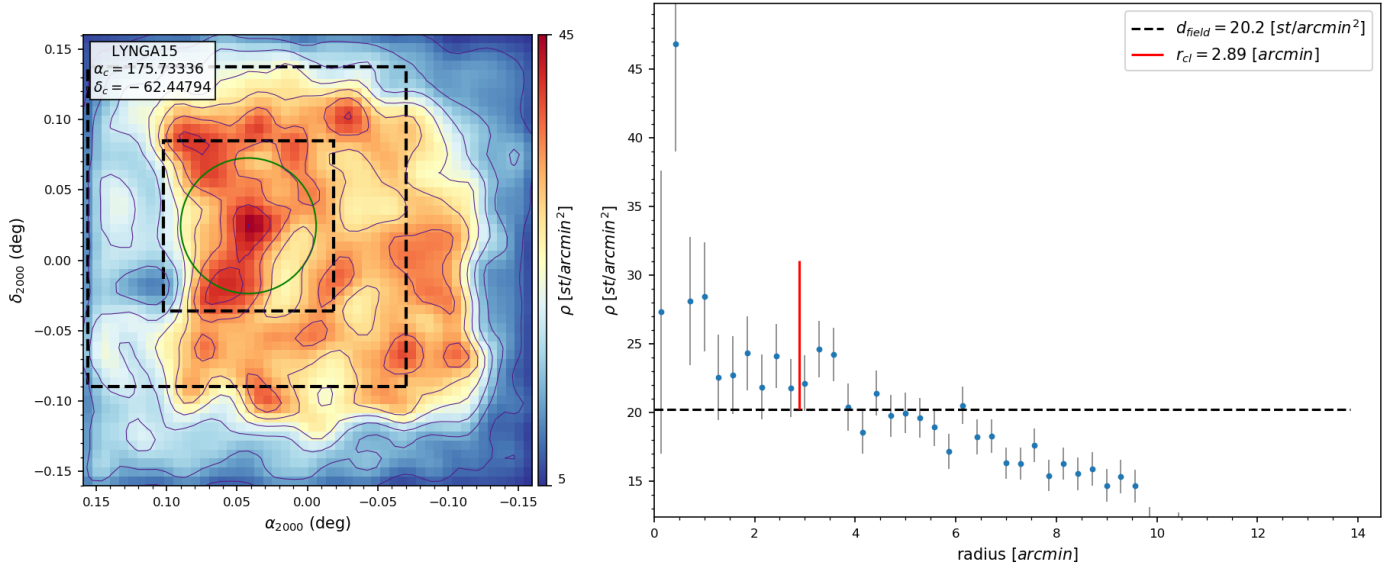
Fig. A.42. Same as Fig. 5 for Lynga 15.
