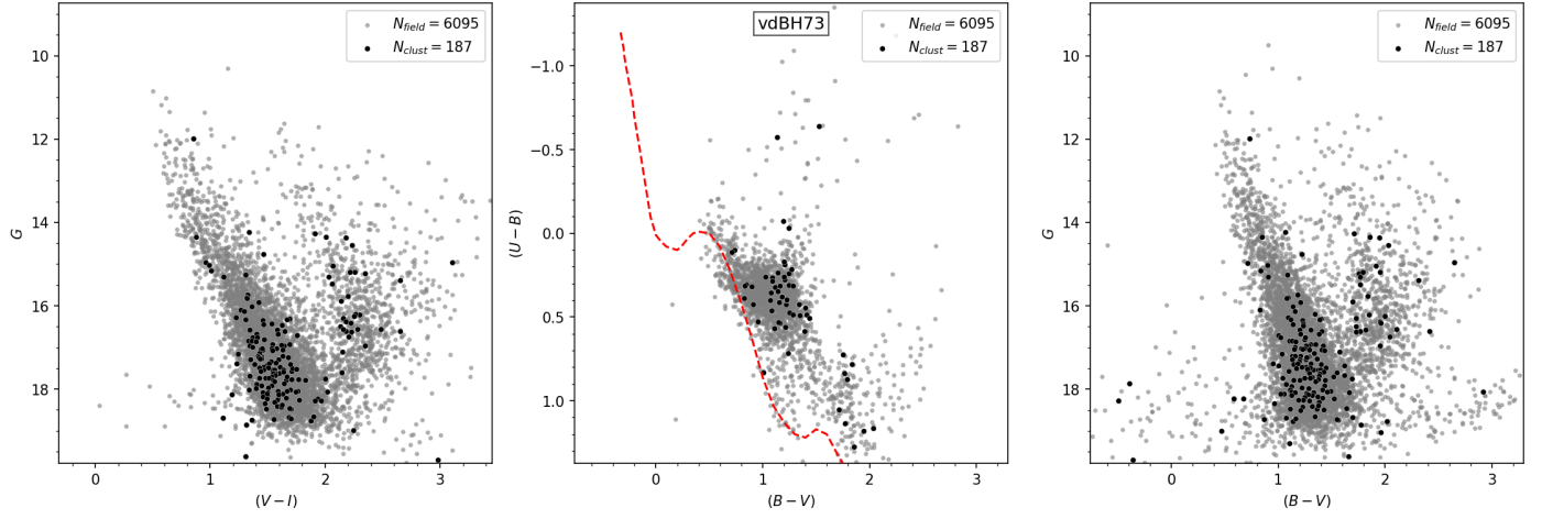
Fig. A.1. Same as Fig. 4 for vdBH 73.
