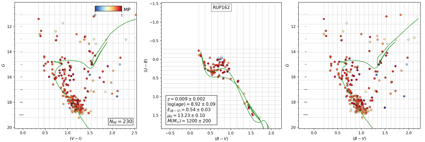
Fig. A.39. Same as Fig. 6 for RUP 162.
