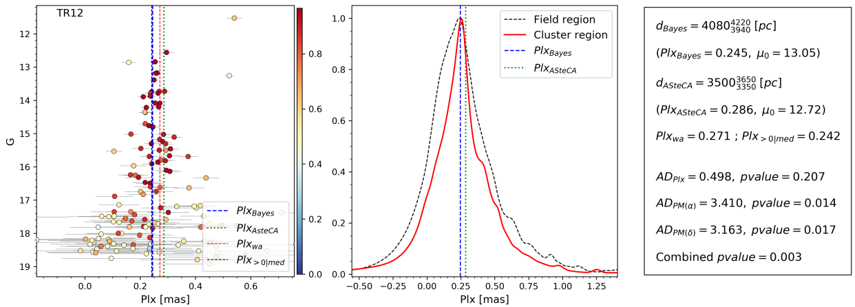
Fig. A.20. Same as Fig. 7 for TR 12.
