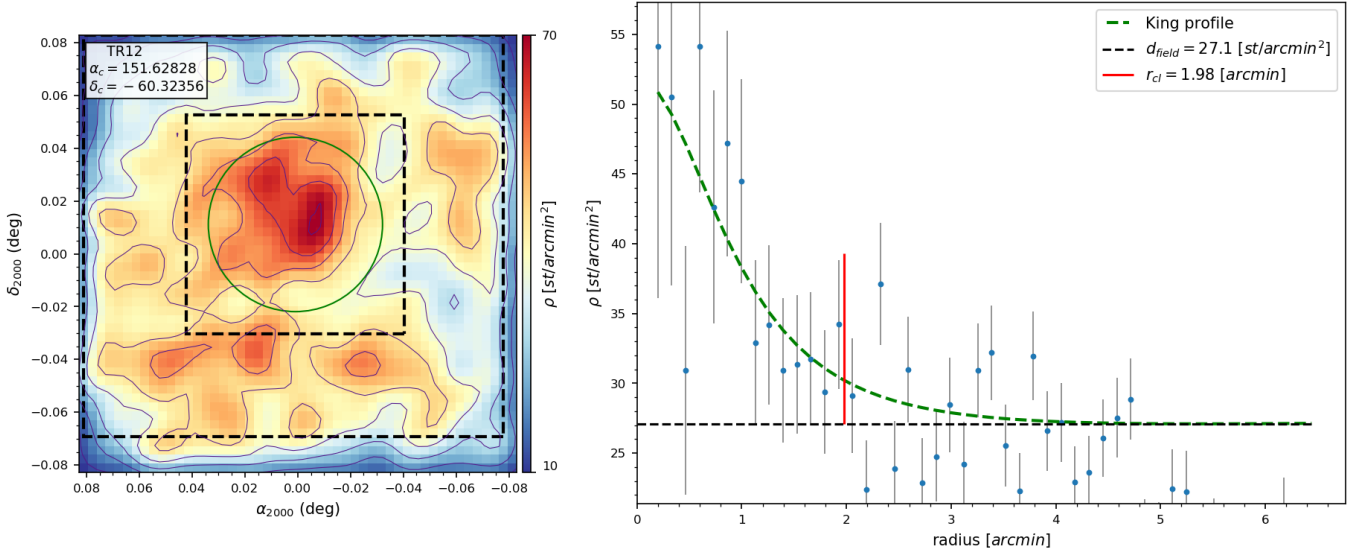
Fig. A.18. Same as Fig. 5 for TR 12.
