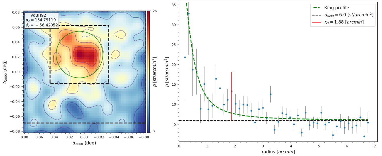
Fig. A.14. Same as Fig. 5 for vdBH 92.
