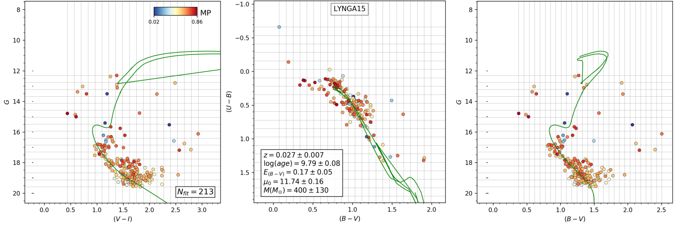
Fig. A.43. Same as Fig. 6 for Lynga 15.
