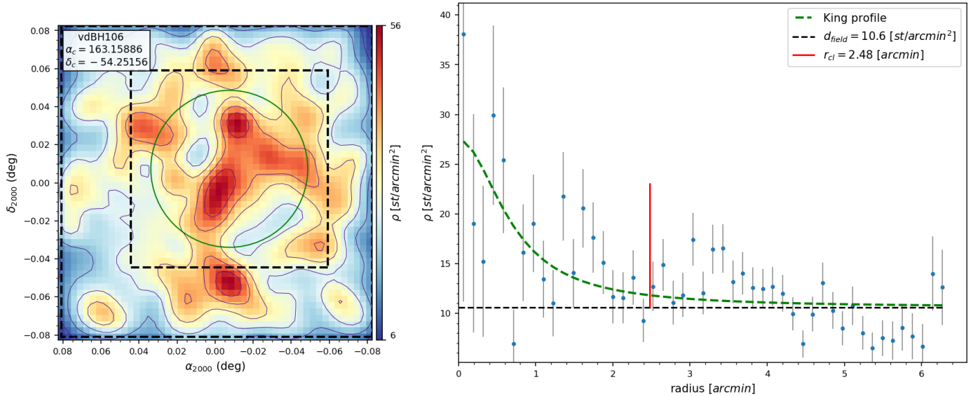
Fig. A.30. Same as Fig. 5 for vdBH 106.
