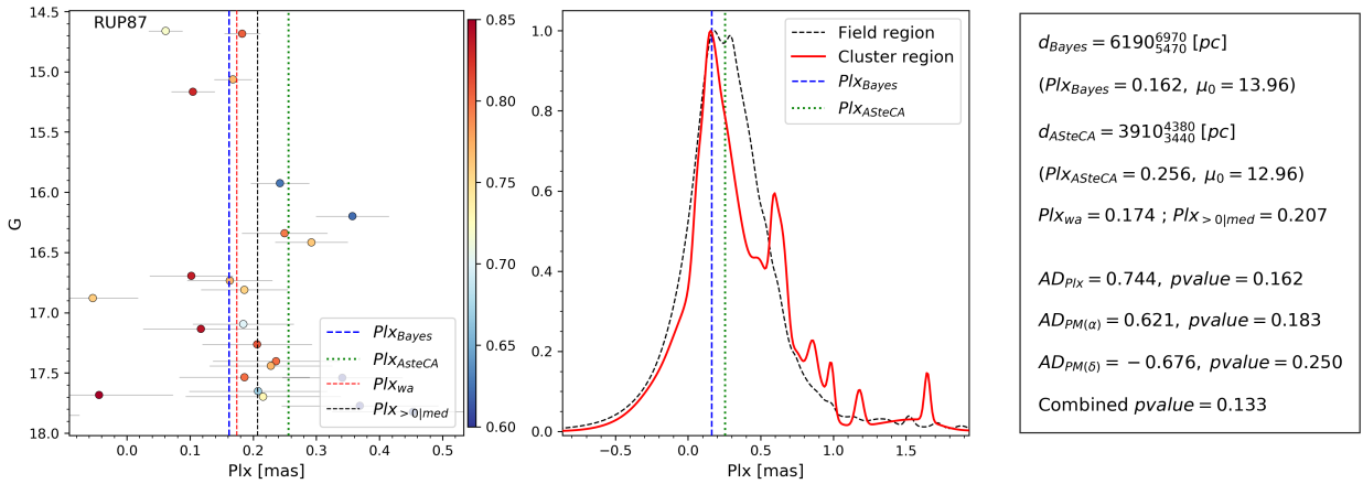
Fig. 15. Same as Fig. 7 for RUP 87.
