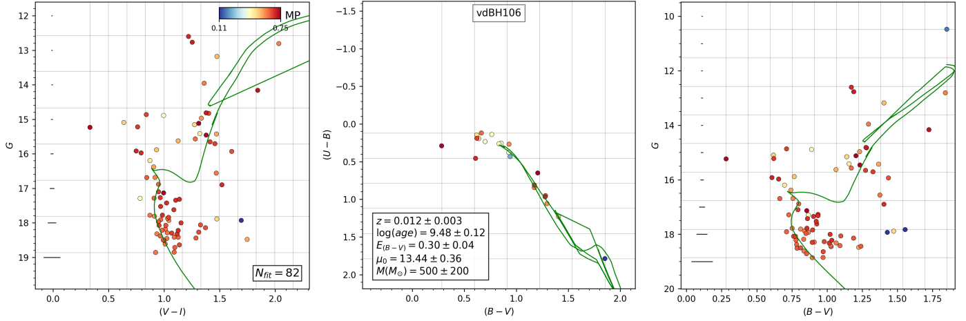
Fig. A.31. Same as Fig. 6 for vdBH 106.
