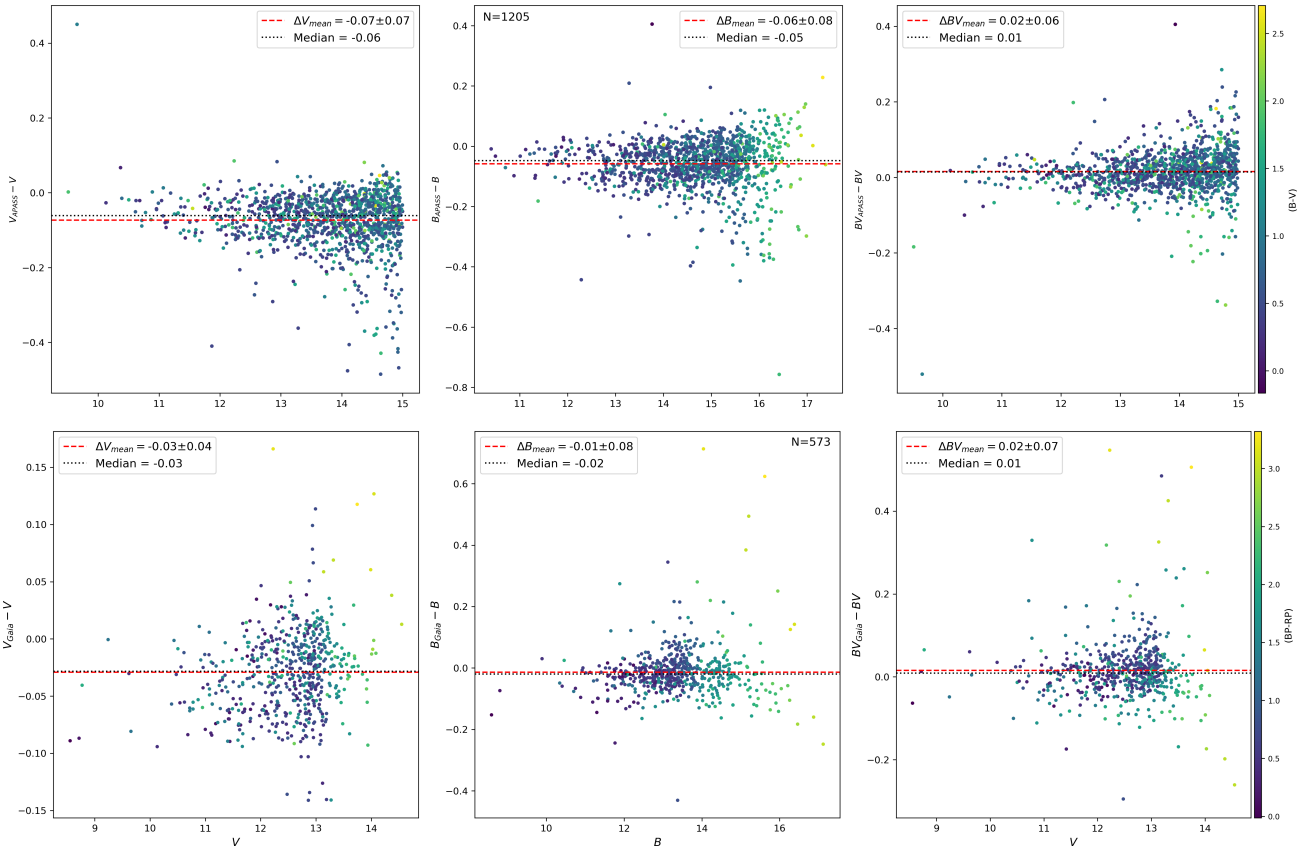
Fig. 2. Top row: differences between the APASS DR10 data for the V (left), B (center) magnitudes and (B - V) color (right) and our own photometry. Bottom row: same for Gaia DR2 data vs. our photometry. Details in the text.
