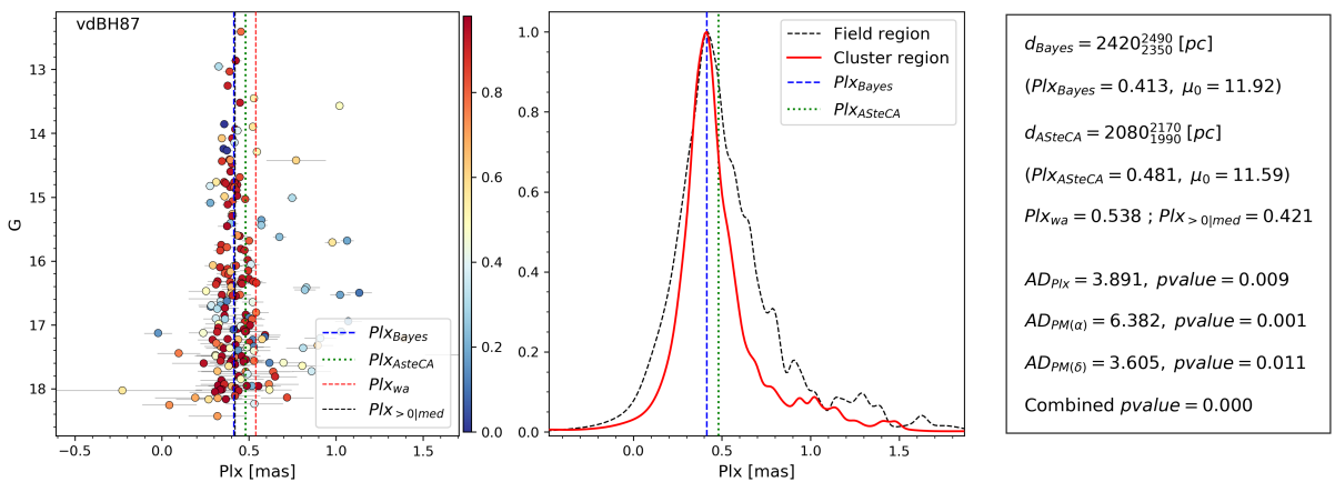
Fig. A.12. Same as Fig. 7 for vdBH 87.
