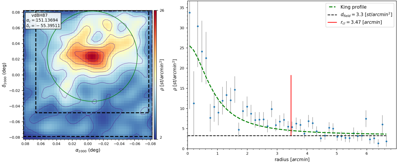
Fig. A.10. Same as Fig. 5 for vdBH 87.
