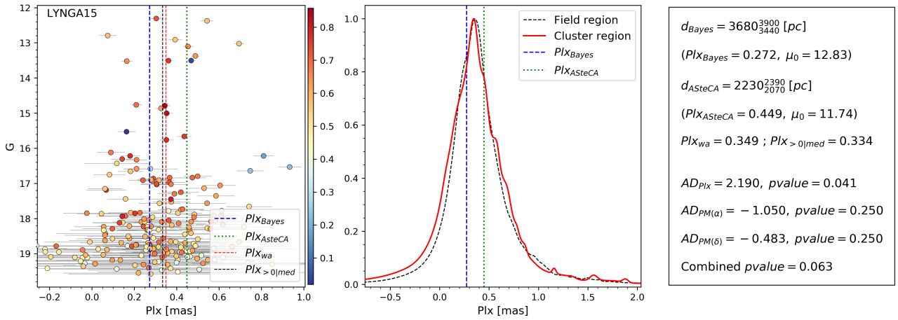
Fig. A.44. Same as Fig. 7 for Lynga 15.
