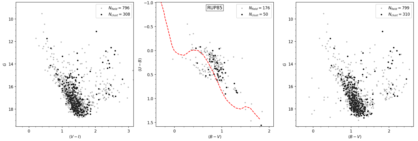
Fig. A.5. Same as Fig. 4 for RUP 85.
