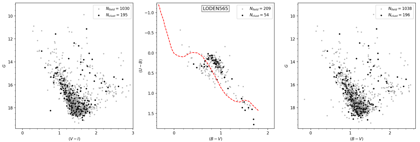
Fig. A.45. Same as Fig. 4 for Loden 565.
