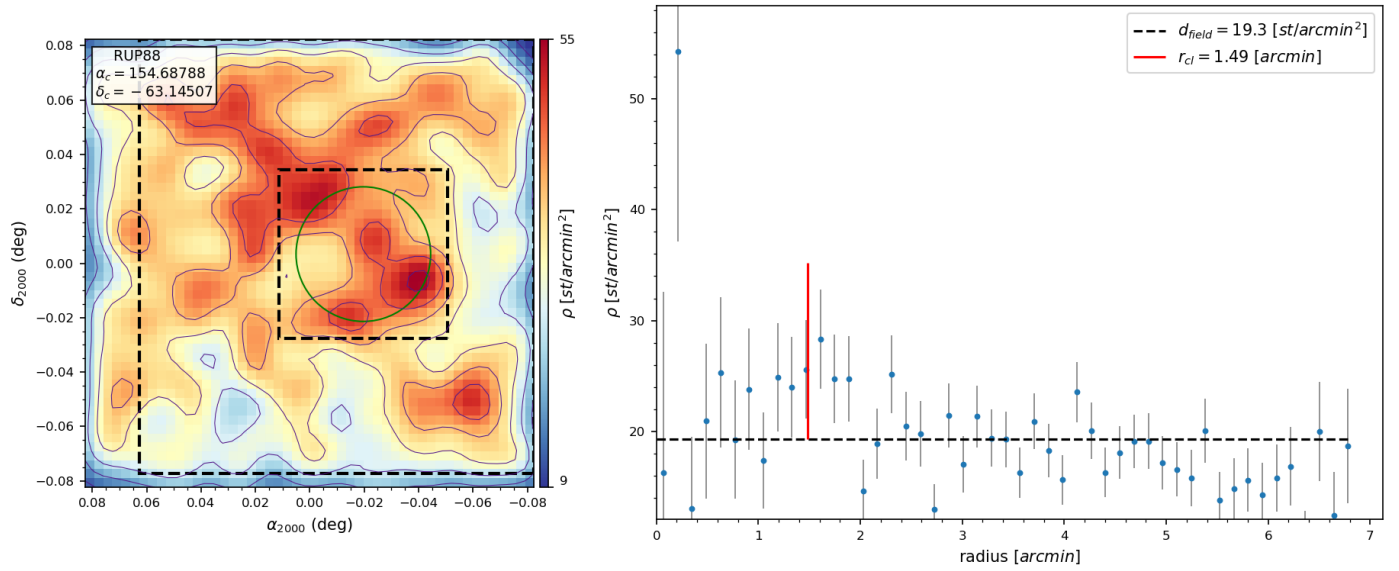
Fig. A.34. Same as Fig. 5 for RUP 88.
