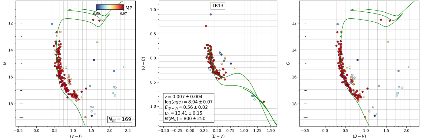
Fig. A.27. Same as Fig. 6 for TR 13.
