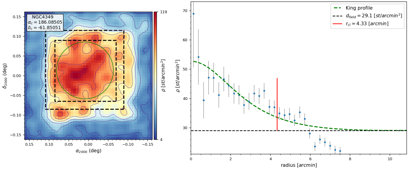
Fig. 9. Same as Fig. 5 for NGC 4349.
