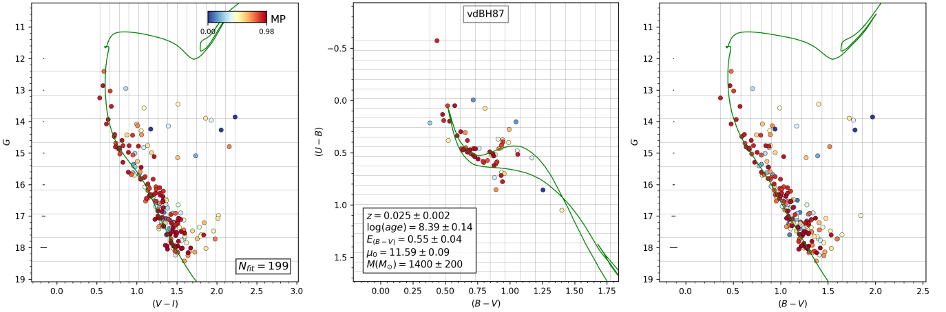
Fig. A.11. Same as Fig. 6 for vdBH 87.
