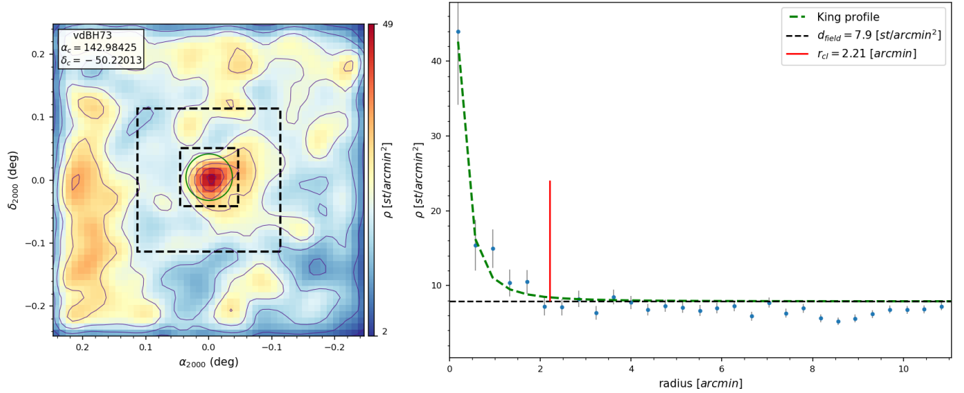
Fig. A.2. Same as Fig. 5 for vdBH 73.
