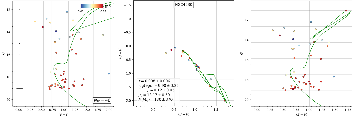
Fig. A.51. Same as Fig. 6 for NGC 4230.
