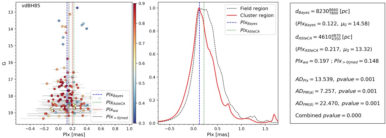
Fig. 7. Left panel: distribution of the parallax for all stars with membership probabilities in the cleaned cluster region as a function of the apparent magnitude G (the vertical color scale shows the membership probability of the star) in vdBH 85. Horizontal bars represent the parallax errors as given by Gaia . The different parallax value fittings are shown by dashed lines of different colors: blue shows the Bayesian parallax estimate, green the AStECA photometric distance, red the weighted average, and black the median (without negative values). Middle panel: normalized comparison between the parallax distributions inside (red line) and outside (dashed black line) the cluster region. The frame at the right summarizes the distances in parsecs according to the Bayesian analysis ( d_{\text{Bayes}} ) and AStECA ( d_{\text{AStECA}} ), followed by the corresponding parallax value, Plx , and corrected distance modulus ( \mu_0 ). Both fittings are indicated by the vertical blue and green dashed lines. The last four text lines in the right panel list the AD values for Plx , PM(\alpha) , and PM(\delta) , followed by the corresponding p -values, and finally, the combined p -value.
