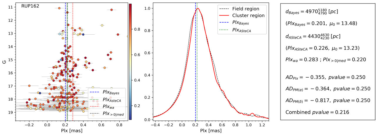
Fig. A.40. Same as Fig. 7 for RUP 162.
