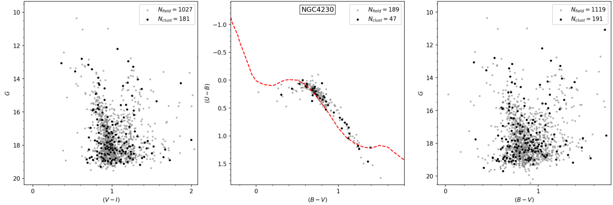
Fig. A.49. Same as Fig. 4 for NGC 4230.
