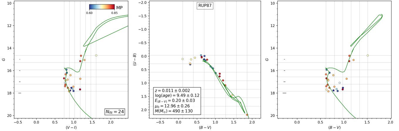
Fig. 14. Same as Fig. 6 for RUP 87.
