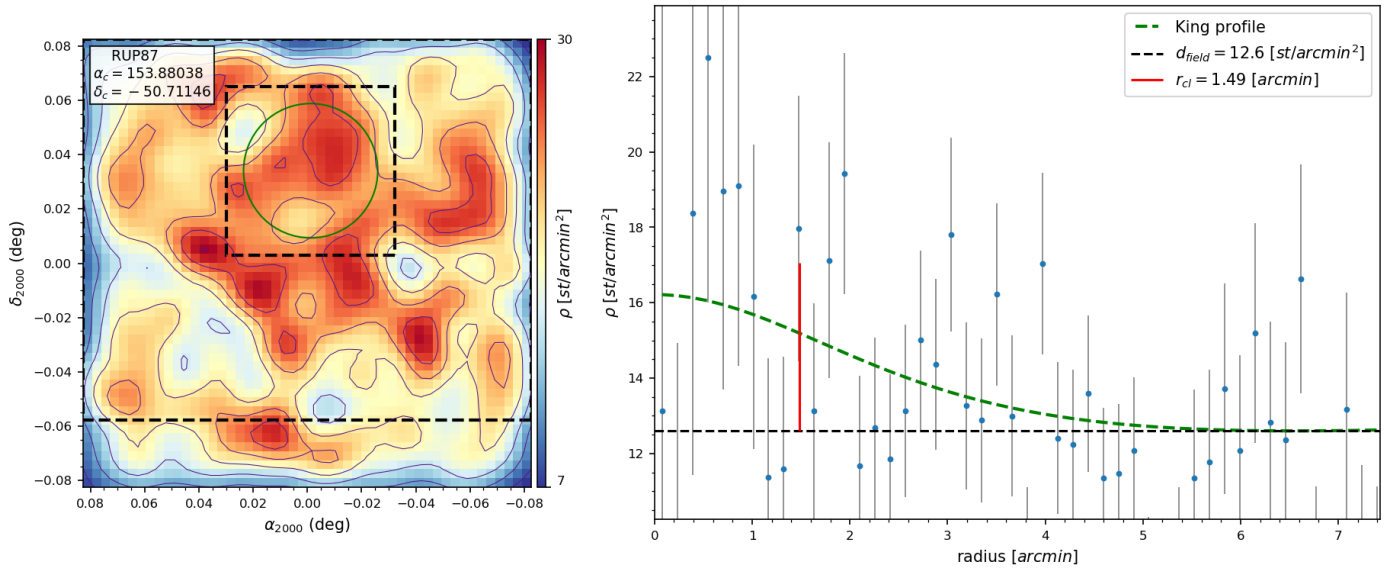
Fig. 13. Same as Fig. 5 for RUP 87.
