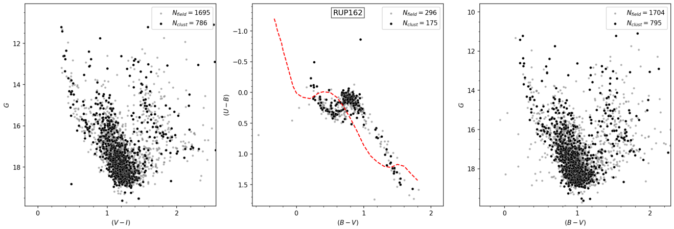
Fig. A.37. Same as Fig. 4 for RUP 162.
