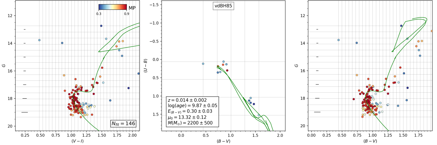
Fig. 6. From left to right: G vs. (V - I) , (B - V) vs. (U - B) , and G vs. (B - V) clean diagrams after field interlopers were removed by AStECA over vdBH 85. The color of each star reflects its membership probability (MP). Corresponding values are in the color bar at the upper right corner in the G vs. (V - I) diagram (left) labeled MP. The CCD in the middle always shows fewer stars because of the U filter. The grid lines trace the edges of the three-dimensional photometric histograms we used to evaluate the likelihood function described in Sect. 4.2. The inset in the lower right corner in the G vs. (V - I) diagram shows the number of stars used by AStECA to compare with synthetic clusters. The inset in the middle panel includes the final results for metallicity, \log(\text{age}) , E(B - V) , the corrected distance modulus, and the total cluster mass provided by AStECA. The green continuous line in the three diagrams is a reference isochrone. In particular, the green line in the CCD, middle panel, shows the most probable E(B - V) value fitting found by AStECA.
