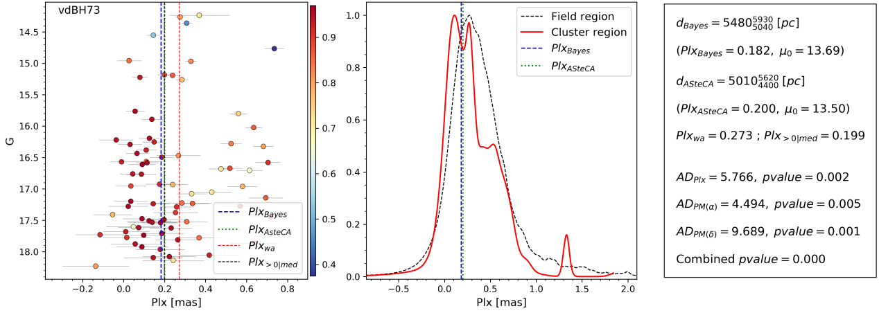
Fig. A.4. Same as Fig. 7 for vdBH 73.
