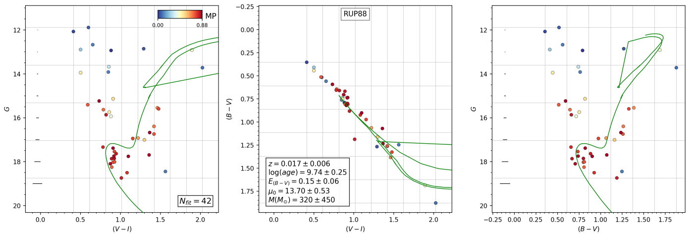
Fig. A.35. Same as Fig. 6 for RUP 88 with the (B - V) vs. (V - I) diagram instead of the (B - V) vs. (U - B) diagram.
