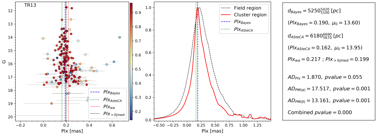
Fig. A.28. Same as Fig. 7 for TR 13.
