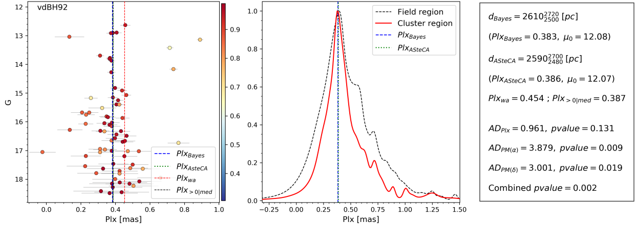
Fig. A.16. Same as Fig. 7 for vdBH 92.
