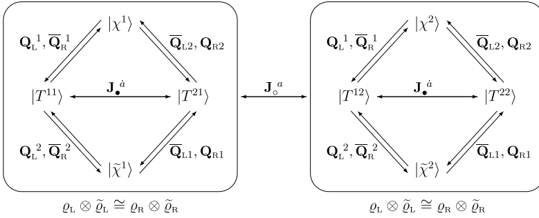
Fig. 2. The massless excitations transform in two irreducible representations of \mathfrak{psu}(1|1)_{\text{c.e.}}^4 , which form a doublet under \mathfrak{su}(2)_\circ . Each of these representation can equivalently be taken to be the massless limit of a left or a right representation with a fermionic highest-weight state. For definiteness, here we take both of them to be given by left representations. Below each \mathfrak{psu}(1|1)_{\text{c.e.}}^4 diagram we indicate how each representation can be obtained from one of two (left or right) isomorphic tensor products of fundamental \mathfrak{su}(1|1)_{\text{c.e.}}^2 representations, see Section 3.1.3.
