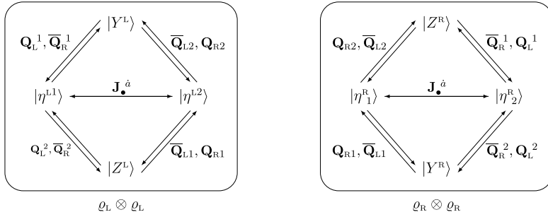
Fig. 1. The massive excitations and their transformation properties under \mathcal{A} . The left and right panel depict the left and right representations respectively. The bosons Z^{L,R} are excitations on \text{AdS}_3 while Y^{L,R} are excitations on S^3 . Note that the massive fermions \eta^{L\dot{a}}, \eta^{R\dot{a}} are charged under \mathfrak{su}(2)_\bullet . The tensor products below each diagram indicate how each representation can be obtained from the short fundamental representations of \mathfrak{su}(1|1)_{\text{c.e.}}^2 introduced in Section 3.1.3.
