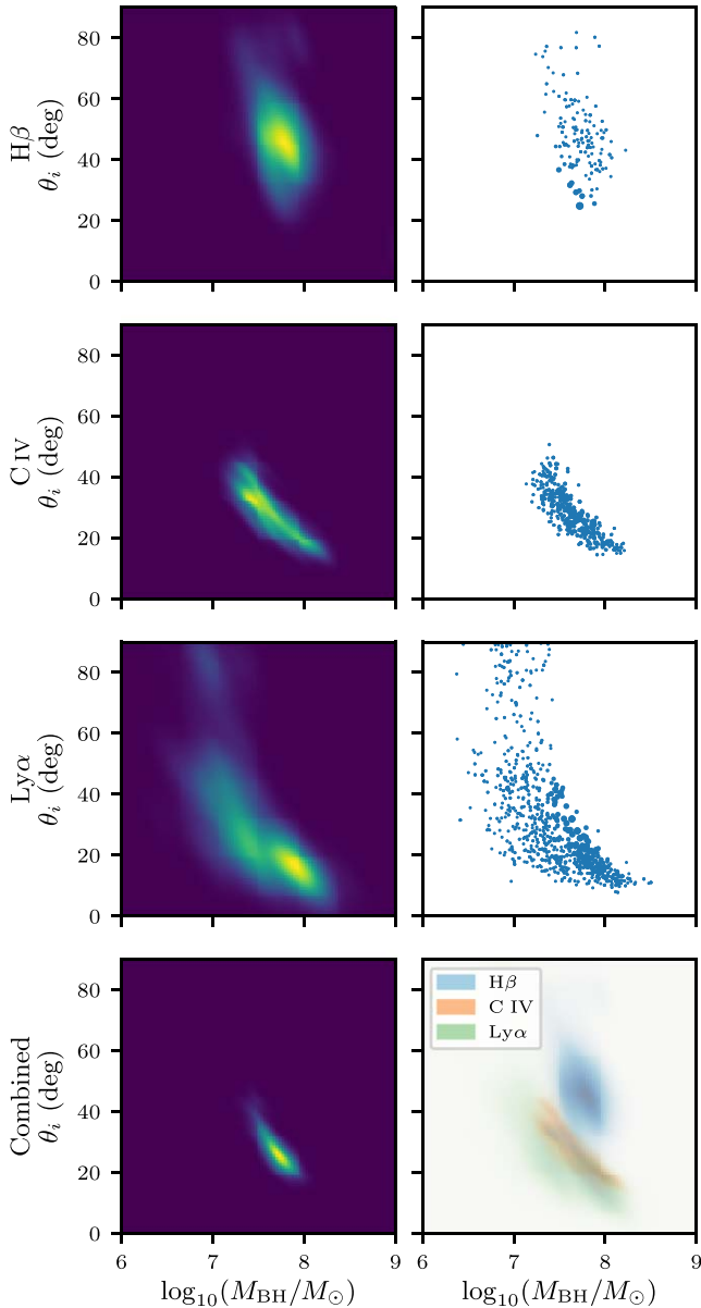
Figure 16. Left: Gaussian kernel density estimates for the 2D posterior probability density functions (PDFs) for (\log_{10}(M_{\text{BH}}/M_{\odot}), \theta_i) in each BLR model as well as the joint constraint (bottom). Right: weighted posterior samples for the three BLR models (top 3), and the region of overlap of the PDFs in the left column (bottom). The size of each point corresponds to the sample’s weight. The weighting scheme used is the one described in Section 5.2 in which the black hole masses and inclination angles for all three BLR models are forced to be the same.
