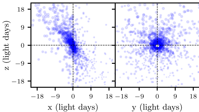
Figure 11. Same as Figure 2, but for the Ly \alpha -emitting BLR.
