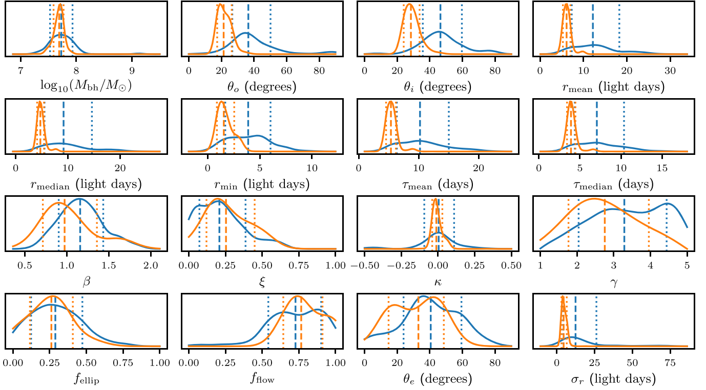
Figure 17. Same as Figure 13, for the H\beta BLR models, but when both M_{\text{BH}} and \theta_i are forced to be the same as those inferred by the \text{Ly}\alpha and C IV models (described in Section 5.2).
