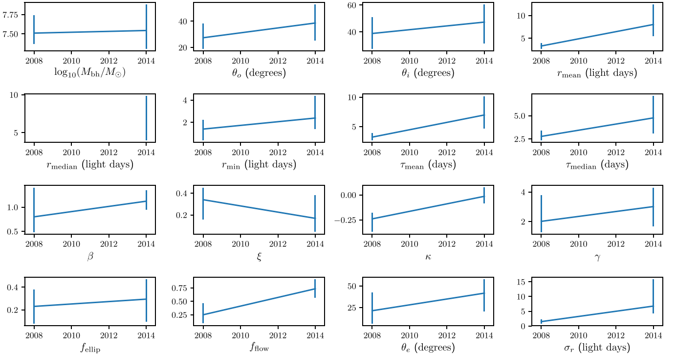
Figure 18. Change in the H\beta BLR model parameters from the LAMP 2008 campaign to the AGN STORM campaign. The vertical bars indicate the posterior PDF median and 68% confidence intervals for the two campaigns. The value of r_{\text{median}} is missing for the 2008 campaign since it was not reported by Pancoast et al. (2014b).
