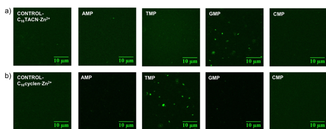
Figure 3. Fluorescence confocal images taken 20 min after mixing a) A or b) B and either one of the nucleotides. Experimental conditions: Amphiphile (30 \mu\text{M} ), coumarin C153 (2.5 \mu\text{M} ) and NMP (30 \mu\text{M} ). Experimental conditions: [HEPES] = 5 mM, pH 7.0, T = 25^\circ\text{C} .
