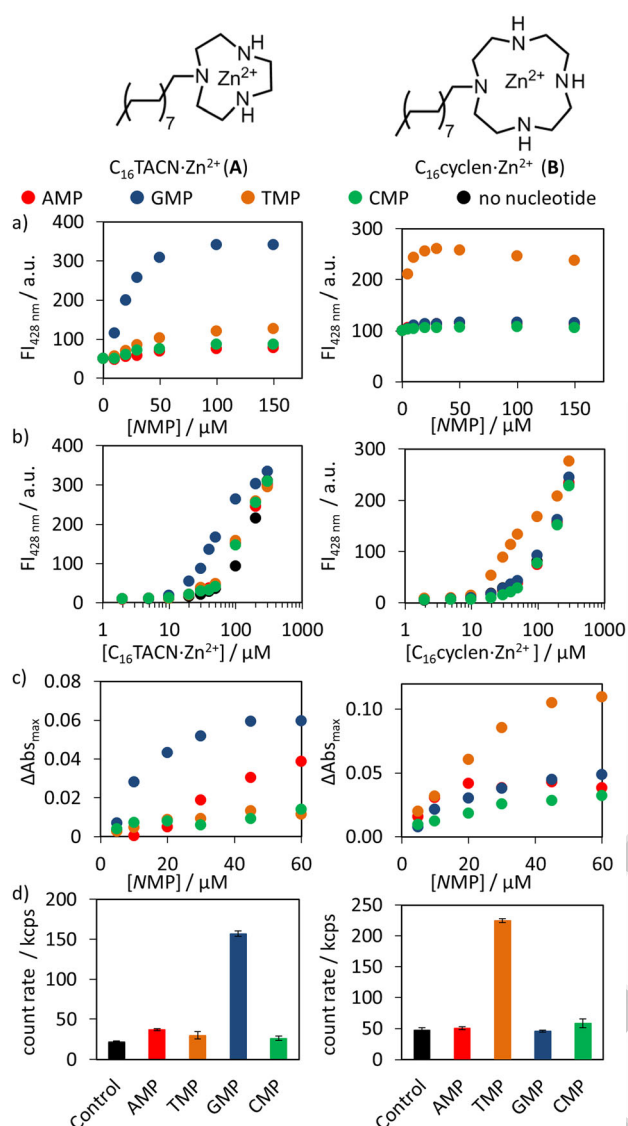
Figure 2. Fluorescence intensity at 428 nm (a) as a function of the NMP concentration ( N = G, T, A, \text{ or } C ) at a fixed amphiphile concentration of 30\ \mu\text{M} A (left graph) or B (right graph) in the presence of DPH ( 2.5\ \mu\text{M} ) and (b) as a function of the amount of amphiphile added (left graph: \text{C}_{16}\text{TACN}\cdot\text{Zn}^{2+} ( A ), right graph: \text{C}_{16}\text{cyclen}\cdot\text{Zn}^{2+} ( B )) to an aqueous buffer solution in the presence of a fixed concentration of NMP ( 30\ \mu\text{M} ). Excitation wavelength = 355\ \text{nm} , slit width (ex/em) = 5/10\ \text{nm} . c) Difference in absorbance at the respective absorbance maxima (AMP = 259\ \text{nm} , TMP = 268\ \text{nm} , GMP = 253\ \text{nm} , CMP = 272\ \text{nm} ) of the nucleotides before and after addition of nucleotides as a function of the nucleotide concentration ( 0\text{--}60\ \mu\text{M} ) added to a solution of amphiphile ( 30\ \mu\text{M} ) (left graph: \text{C}_{16}\text{TACN}\cdot\text{Zn}^{2+} ( A ), right graph: \text{C}_{16}\text{cyclen}\cdot\text{Zn}^{2+} ( B )). d) Scattering intensity rate (count rate, kcps) measured by dynamic light scattering (DLS) of the aggregates formed in the absence and presence of NMPs ( 30\ \mu\text{M} ) and a fixed amount of surfactant ( 30\ \mu\text{M} ) (left graph: \text{C}_{16}\text{TACN}\cdot\text{Zn}^{2+} ( A ), right graph: \text{C}_{16}\text{cyclen}\cdot\text{Zn}^{2+} ( B )). All measurements were performed in triplicate. Experimental conditions: [\text{HEPES}] = 5\ \text{mM} , \text{pH } 7.0 , T = 25\ ^\circ\text{C} .
