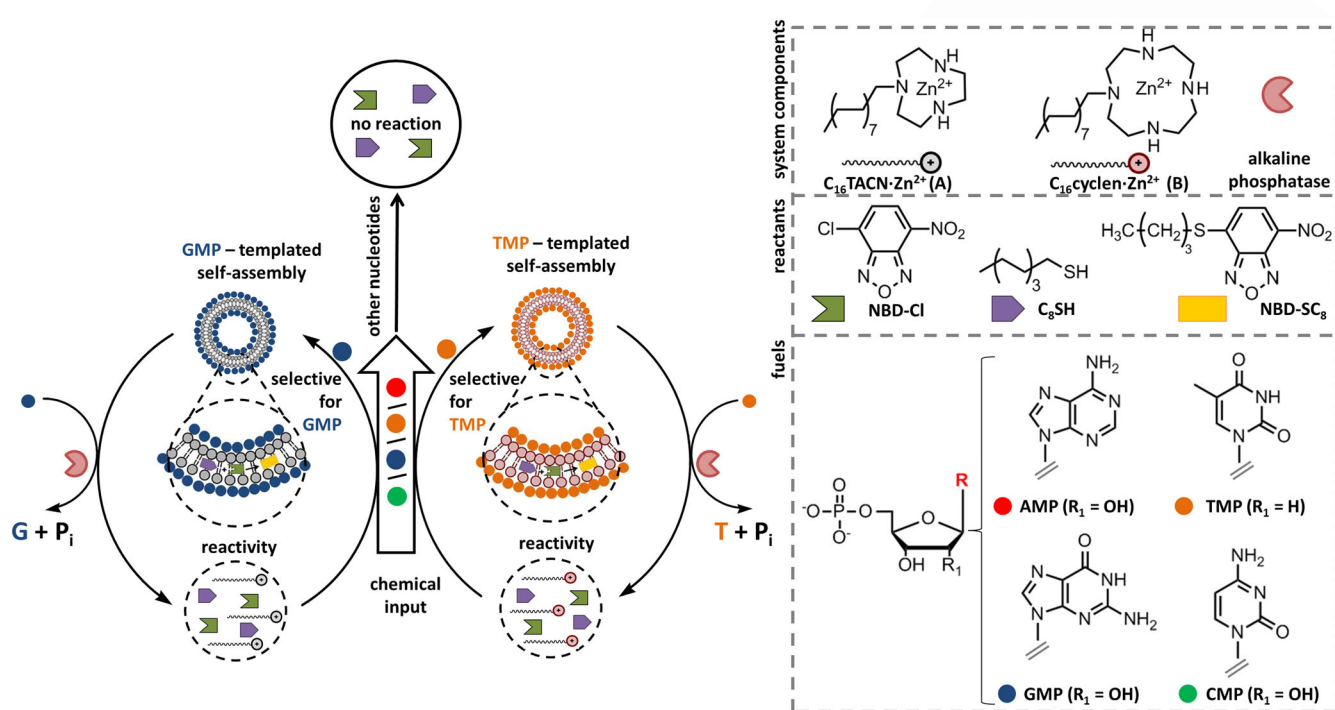
Figure 1. Schematic representation of nucleotide-selective templated self-assembly of nanoreactors under dissipative conditions and consequent transient activation of a chemical reaction between C_8SH and NBD-Cl.
