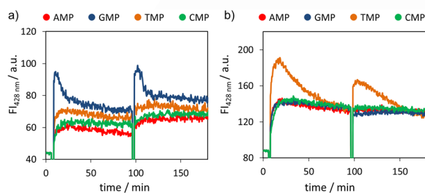
Figure 5. Fluorescence intensity at 428 nm following two repetitive additions of NMP (30 \mu\text{M} ; N = A, T, G, C) to a solution of a) A (30 \mu\text{M} ) or b) B (30 \mu\text{M} ) and DPH (2.5 \mu\text{M} ) in the presence of alkaline phosphatase (AP) (1 \text{U mL}^{-1} ). Experimental conditions: [HEPES] = 5 mM, pH 7, T = 25^\circ\text{C} .
