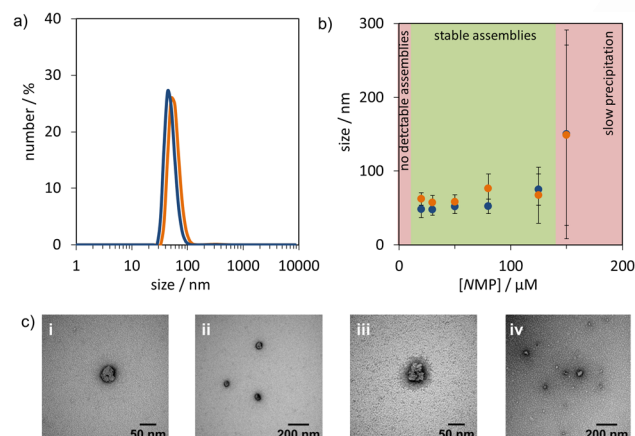
Figure 4. a) Representative DLS graphs of solutions containing A and GMP (30 \mu\text{M} each, blue trace) or B and TMP (30 \mu\text{M} each, orange trace). Experimental conditions: [HEPES] = 5 mM, pH 7, T = 25^\circ\text{C} . b) Hydrodynamic diameters measured with DLS as a function of NMP concentration (10–150 \mu\text{M} ) at a constant amphiphile concentration (30 \mu\text{M} ) in HEPES buffer (pH 7, 5 mM). Blue dots correspond to the A - GMP system and orange dots correspond to B - TMP system. The green area indicates the concentration regime at which stable assemblies were observed. c) TEM images of a solution containing NMP (30 \mu\text{M} ) and amphiphile (30 \mu\text{M} ) in HEPES buffer (pH 7, 5 mM). i–ii) TEM images of A - GMP , iii–iv) TEM images of B - TMP . Samples were stained with 2% uranyl acetate solution.
