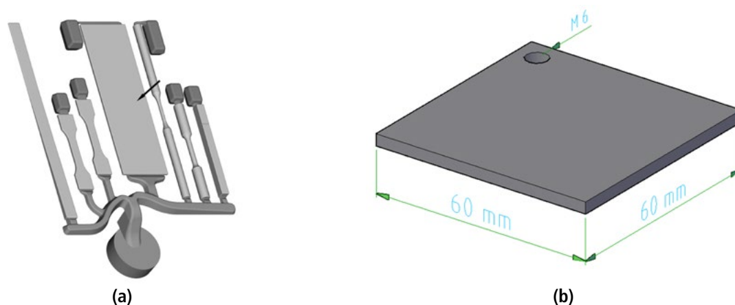
Fig. 1 – (a) Geometry of the die-casting, where the investigated plate is indicated by arrow; (b) dimensions of the drawn specimen that was hard-anodized and analysed in the present work.
