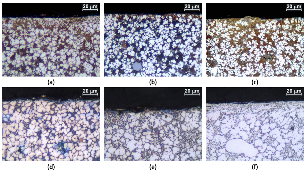
Fig. 3 – Typical etched microstructures of diecast (a,d) AlSi9Cu3(Fe), (b,e) AlSi11Cu2(Fe) and (c,f) AlSi12Cu1(Fe) alloys. The micrographs refer to (a,b,c) as-diecast and (d,e,f) milled surfaces.
