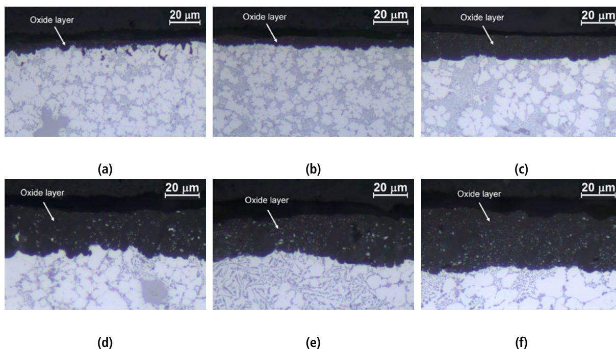
Fig. 4 – Anodic oxide layer formed on diecast (a,d) AlSi9Cu3(Fe), (b,e) AlSi11Cu2(Fe) and (c,f) AlSi12Cu1(Fe) alloy surfaces. The micrographs refer to the (a,b,c) as-diecast and (d,e,f) milled substrates.
