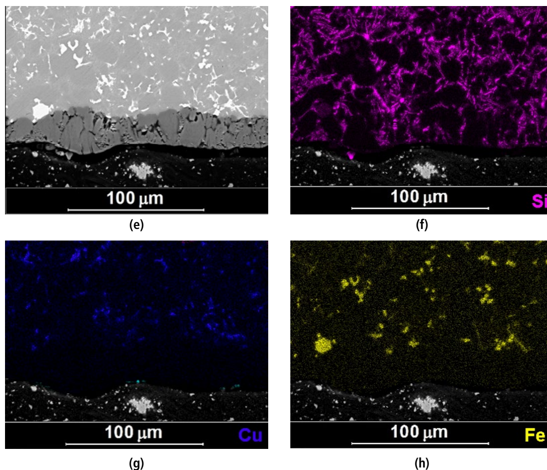
Fig. 6 – FEG-SEM micrographs of the anodic oxide layer with the corresponding EDS composition maps showing the distribution of Si, Cu and Fe elements in (a-d) as-diecast and (e-h) milled AlSi9Cu3(Fe) alloy surfaces.
