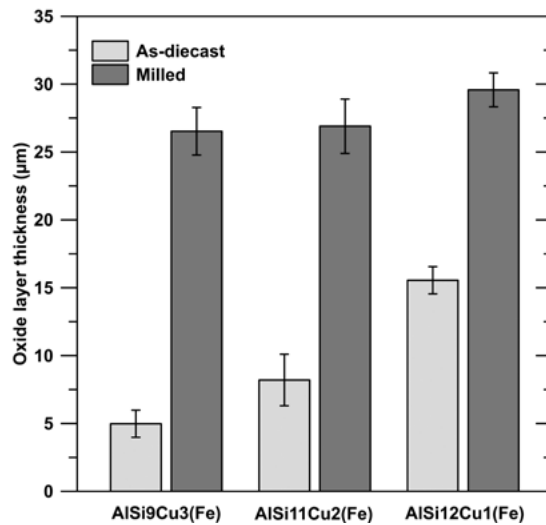
Fig. 5 – Thickness of the anodic oxide layer as function of the alloy composition and finishing condition. The scattering of data is depicted by vertical bars.
