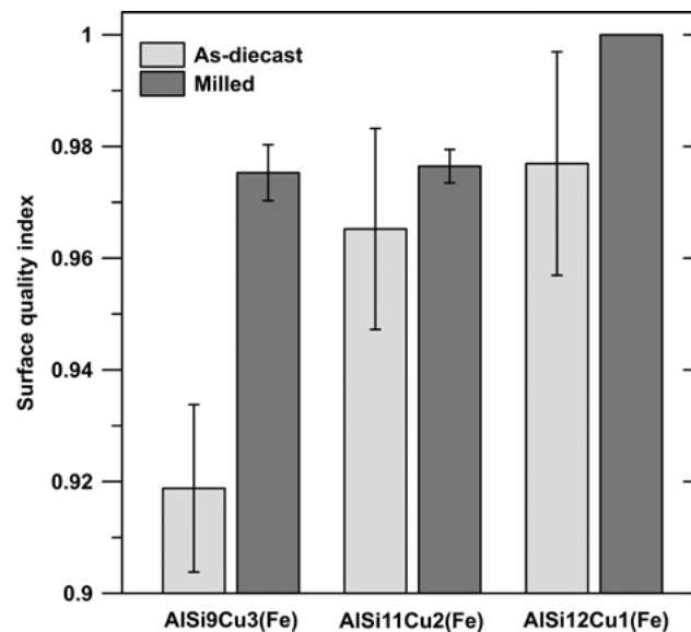
Fig. 7 – Variation of the surface quality of hard anodized surfaces in the different experimental conditions; the quality was evaluated by means of the surface quality index defined in §2.4.
