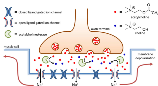
Figure 6. Schematic representation of a synaptic cleft at a neuromuscular junction. Acetylcholine is released from vesicles in the axon terminal and causes opening of ligand-gated ion channels in the muscle cell. At the same time, acetylcholine is rapidly cleared from the synaptic cleft by the enzyme acetylcholinesterase.
