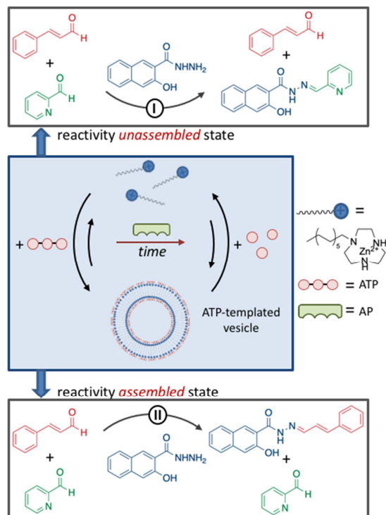
Figure 7. ATP-templated self-assembly of vesicles under dissipative conditions installed by the presence of the enzyme alkaline phosphatase. The assembly state affects the chemical reactivity in the system: reaction I dominates in the unassembled state, whereas reaction II dominates in the assembled state. Transient inversion of reaction selectivity is observed upon the addition of ATP.
