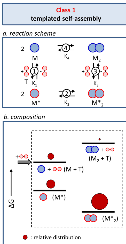
Figure 2. Class 1 - Templated self-assembly. a) The reaction scheme describes the chemical connectivity between the components of the system. b) Energy diagram in which the dark red circles indicate the composition of the system in the presence of template T .
