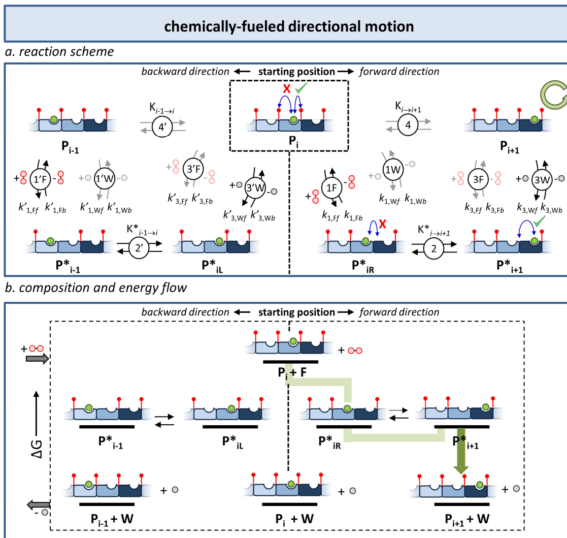
Figure 14. Chemically-fueled unidirectional motion. a) Model used to illustrate how kinetic asymmetry leads to unidirectional motion. b) Energy diagram that serves to explain how energy dissipation leads to motion in the forward direction. The green trajectory represents the preferential energy dissipation pathway leading to motion in the forward direction. The dark green coloured arrow represents the step in which waste molecules are generated.
