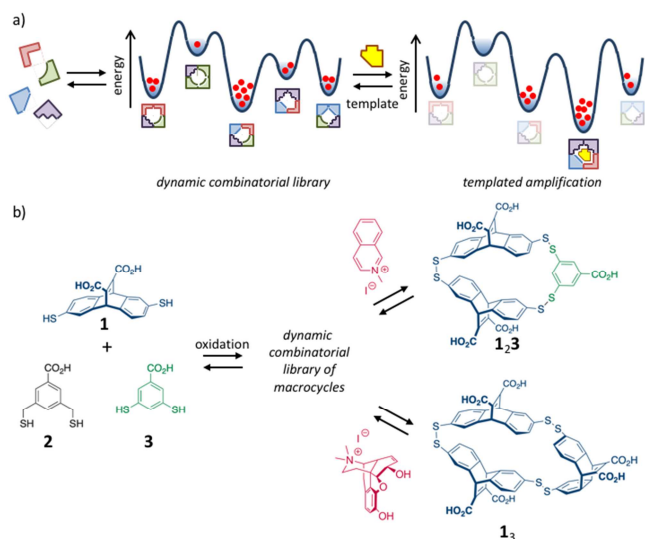
Figure 4. a) Schematic representation of the formation of a dynamic combinatorial library from a mixture of building blocks and the spontaneous adaptation to the addition of a template. b) Mixing building blocks 1 – 3 results in the formation of a dynamic library of macrocycles containing at least 45 distinct structures. The addition of templates causes the selective amplification of library members. [85]
