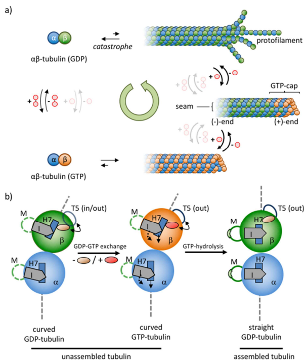
Figure 12. a) GTP-fueled self-assembly of microtubules. b) Structural changes in the \alpha\beta -tubulin dimer as a function of the occupancy of the E-site with GDP or GTP. Conversion of GTP to GDP in assembled tubulin leads to strain in the microtubule lattice. Figure inspired by ref. [144]
