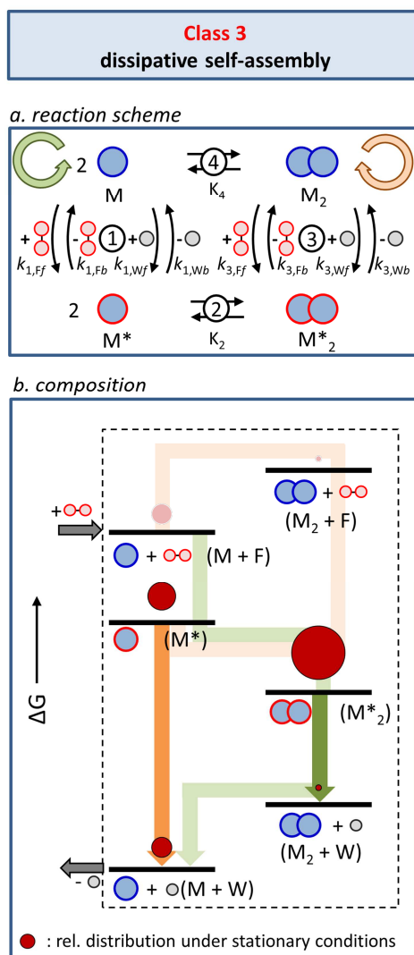
Figure 8. Class 3 - Dissipative self-assembly. a) Class 3 is characterized by the presence of two chemical connectivities between the non-activated and activated building blocks involving either fuel or waste. b) Energy diagram that illustrates the composition of the system under stationary conditions, i.e. at constant fuel and waste concentrations in an open system. The orange and green trajectories represent the clockwise (orange) and counterclockwise (green) directions of the cycle depicted in Figure 8a. The dark coloured arrows correspond to the processes during which waste molecules are generated. The size of the dark red circles indicate the relative populations of the respective states taken from previously reported simulations. [62]
