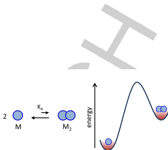
Figure 1. Equilibrium between M and M_2 used as a reference throughout the article. The composition at equilibrium is defined by the equilibrium constant K_4 ( M^{-1} ). The notation for the equilibrium constant – K_4 – is used to facilitate the comparison of the discussion in this work with a previous publication. [62]
