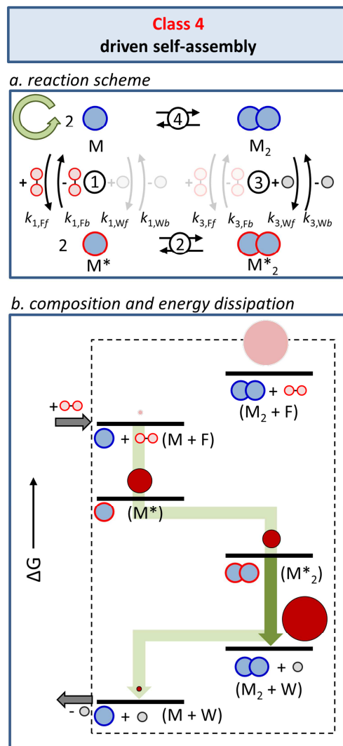
Figure 11. Class 4 - Driven self-assembly. a) Kinetic asymmetry arises from the presence of different energy barriers for the fuel and waste reactions with respect to the unassembled (M) and assembled ( M_2 ) states. b) Energy diagram that illustrates how kinetic asymmetry creates the conditions required for the permanent population of the high-energy assembly M_2 under stationary conditions. The green trajectory represent the counterclockwise (green) direction of the cycle depicted in Figure 11a. The dark green coloured arrow correspond to the process during which waste molecules are generated. The size of the dark red circles indicate the relative population of the respective state taken from previously reported simulations. [62]
