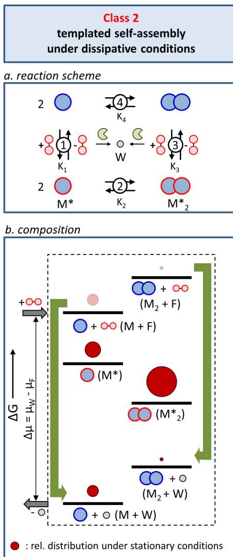
Figure 5. Class 2 - Templated self-assembly under dissipative conditions. a) The reaction scheme describes the chemical connectivity between the components of the system and the energy dissipation process. b) Energy diagram that illustrates the composition of the system under stationary conditions, i.e. at constant fuel and waste concentrations in an open system. The green arrows indicate the energy dissipation steps. The size of the dark red circles indicate the relative populations of the respective states taken from previously reported simulations. [62]
