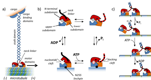
Figure 15. Schematic representation of kinesin-1. b) Structural changes in the motor domain as a function of binding site occupancy by ADP and ATP. c) ATP-fueled directional motion of kinesin towards the (+)-end of a microtubule. Figures b and c are inspired by ref. [159]
