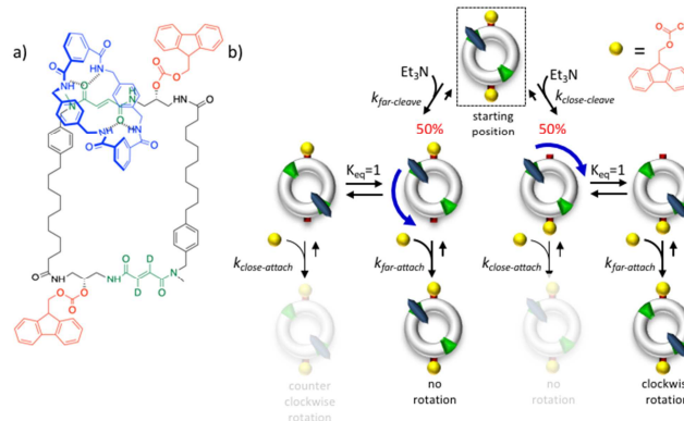
Figure 16. a) Chemical structure of a [2]catenane used for Fmoc-Cl fueled directional rotation of the small ring (blue) around the large ring. b) Illustration of how a single removal-attachment cycle leads to net rotation of the blue ring in a clockwise direction.
