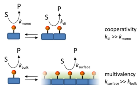
Figure 17. Exploitation of cooperativity and multivalency for the installment of kinetic asymmetry.
