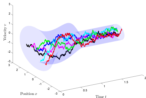
Fig. 5: Inertial particles: trajectories in phase space
