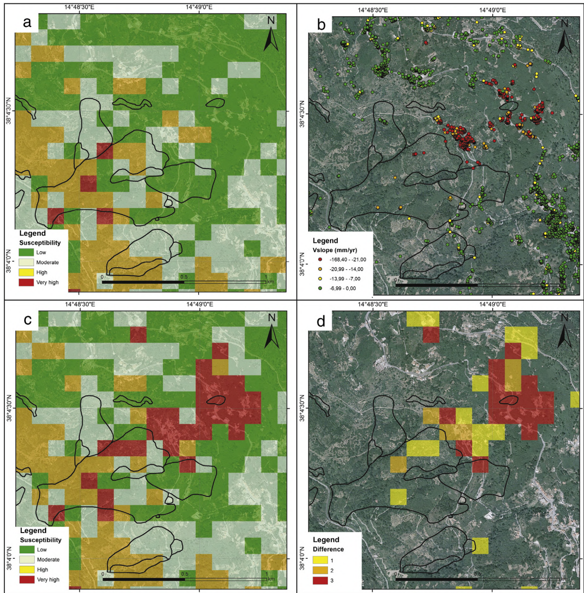
Fig. 11. (a) Original LSM of the Castell'Umberto municipality area; (b) V_{slope} ground deformation velocity map; (c) new LSM obtained after the application of the correction matrix; (d) difference between the original LSM and the new LSM.
