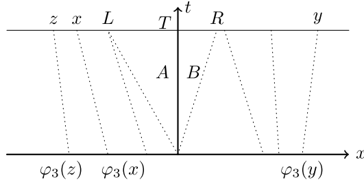
FIGURE 4. Characteristics's behaviour for profiles in \mathcal{A}_3^{AB}(T) .
