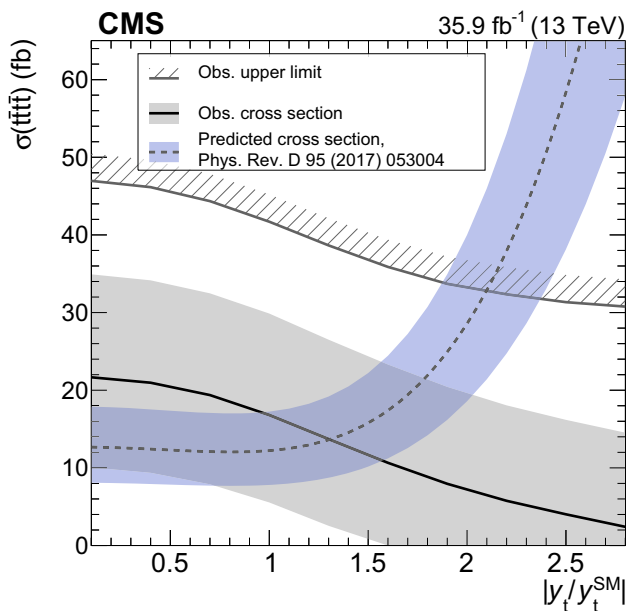
Fig. 5 The predicted SM value of \sigma(pp \rightarrow t\bar{t}\bar{t}) [16], calculated at LO with an NLO/LO K -factor of 1.27, as a function of |y_t/y_t^{\text{SM}}| (dashed line), compared with the observed value of \sigma(pp \rightarrow t\bar{t}\bar{t}) (solid line), and with the observed 95% CL upper limit (hatched line)
