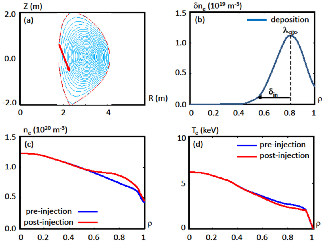
Figure 17. Pellet ablation simulation with the HPI2 code, for Scenario 3, corresponding to the case ‘In 470 \text{m s}^{-1} ’ of table 4. (a) Injection geometry; (b) pellet deposition profile versus normalized radius; (c) pre- and post-injection electron density profiles; (d) the same for the electron temperature.
