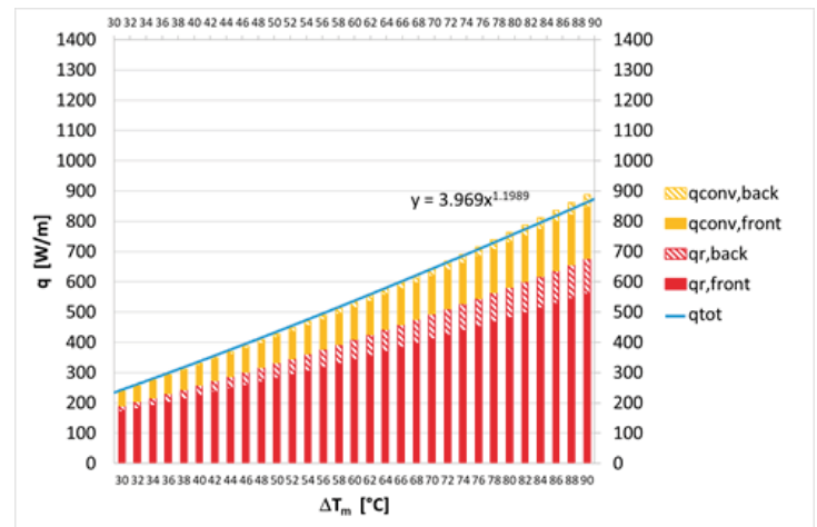
Figure 4 – Thermal power exchanged by the water strip (expressed in watt per meter of linear length of the water strip as it is referred to a strip having 0.9 m width) with no flashing presence and with thermal insulation for the operation conditions of the EN14037 standard
