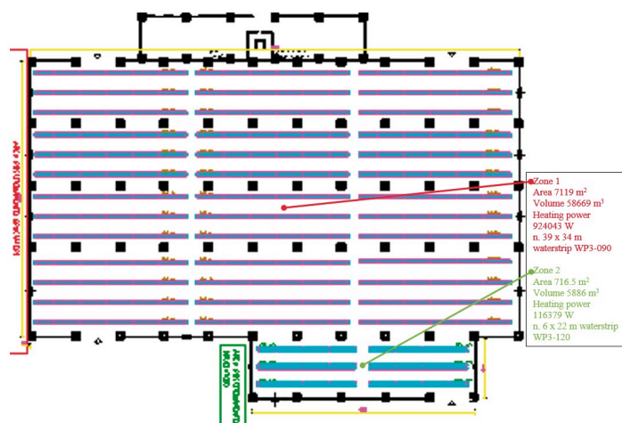
Figure 1 – Factory shed used in the present study (courtesy of Studio di Ingegneria Larovere ing. Marco)
