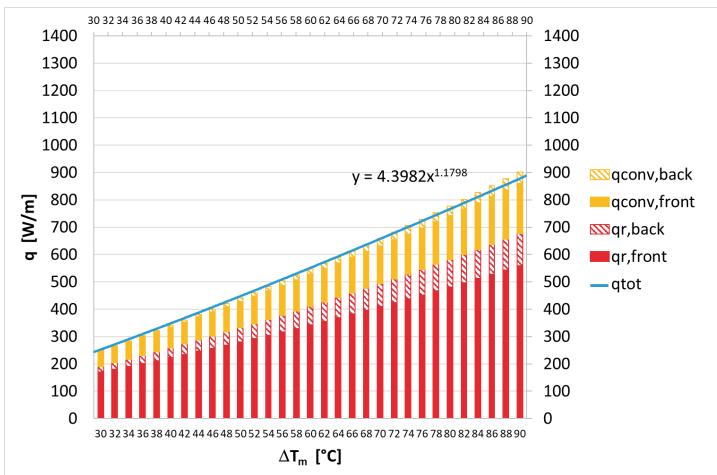
Case 4 – Nat. Conv. – \alpha_{conv,front} = 1.736 \cdot (T_{p,front,avg} - T_{ai})^{0.16} / D_e^{0.52}
