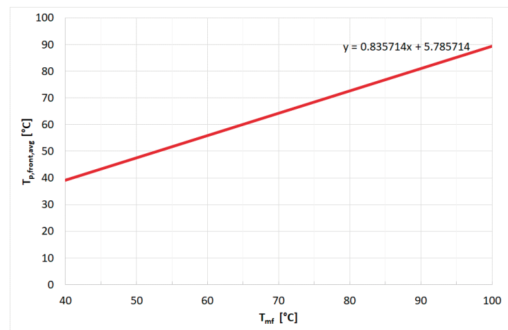
Figure 2 – Front side plate average temperature ( T_{p,front,avg} ) in function of the hot water average temperature ( T_{mf} )
