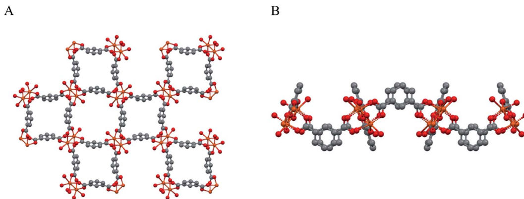
Fig. 3 Sketches of the weakly corrugated 2D layers in the crystal packing of \text{Cu}_2(\mu\text{-isophthalate})_4\text{D}_2 , present also in [\text{Cu}(\text{1,3-YBDC})] \cdot x\text{H}_2\text{O} . (A) View down [001]. (B) View down [100]. Note that, in [\text{Cu}(\text{1,3-YBDC})] \cdot x\text{H}_2\text{O} , the layers are not separated, but are interlinked by the long propargyl carbamate residues (in both a and b conformations) completing the \text{Cu}_2(\mu\text{-COO})_4 coordination sphere (the apical D atom) with a truly 3D connectivity.
