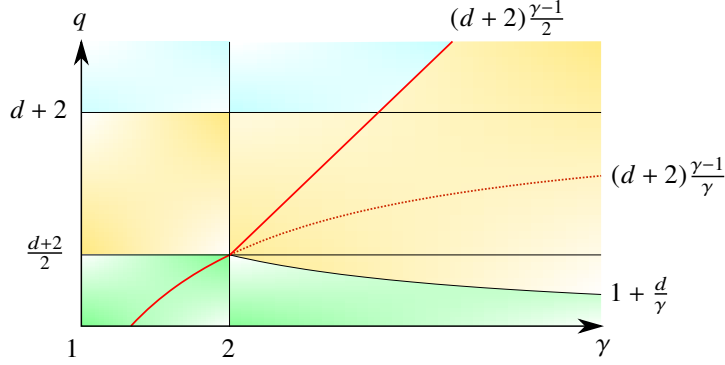
Figure 1: A sketch of estimates that are known for solutions to (HJ), as \gamma and q vary: L^p (green region), Hölder (yellow region), Lipschitz (light blue region, [21]). Above the solid red line we prove here maximal regularity estimates (Theorems 1.1 and 1.3). Above the dashed red line we prove here new Hölder estimates (Theorem 1.2). When \gamma > 2 and 1 + \frac{d}{\gamma} < q < \frac{(d+2)^{\gamma-1}}{2} (yellow zone between the dashed red line and the solid black line) Hölder estimates have been obtained in [14, 66] under sign conditions on the right-hand side, while integrability estimates in the green region below the threshold q = 1 + \frac{d}{\gamma} can be found in [12].
