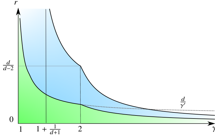
Figure 2: A sketch of regions where existence of classical solutions to (MFG) are obtained, in the monotone case (light blue and green regions) and in the non-monotone case (green region only).
