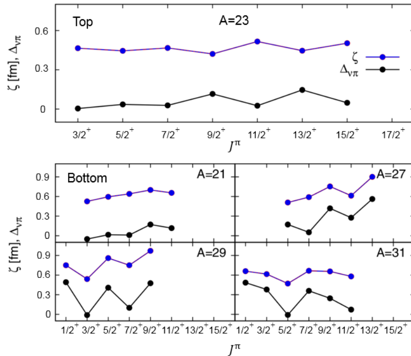
Fig.4 Comparison between the trend of the neutron skin parameter \zeta and the difference in neutron and proton occupation numbers of the s_{1/2} orbital: (a) for the mirror nuclei A=23 ; (b) for the other T=1/2 mirror nuclei in the sd shell.
