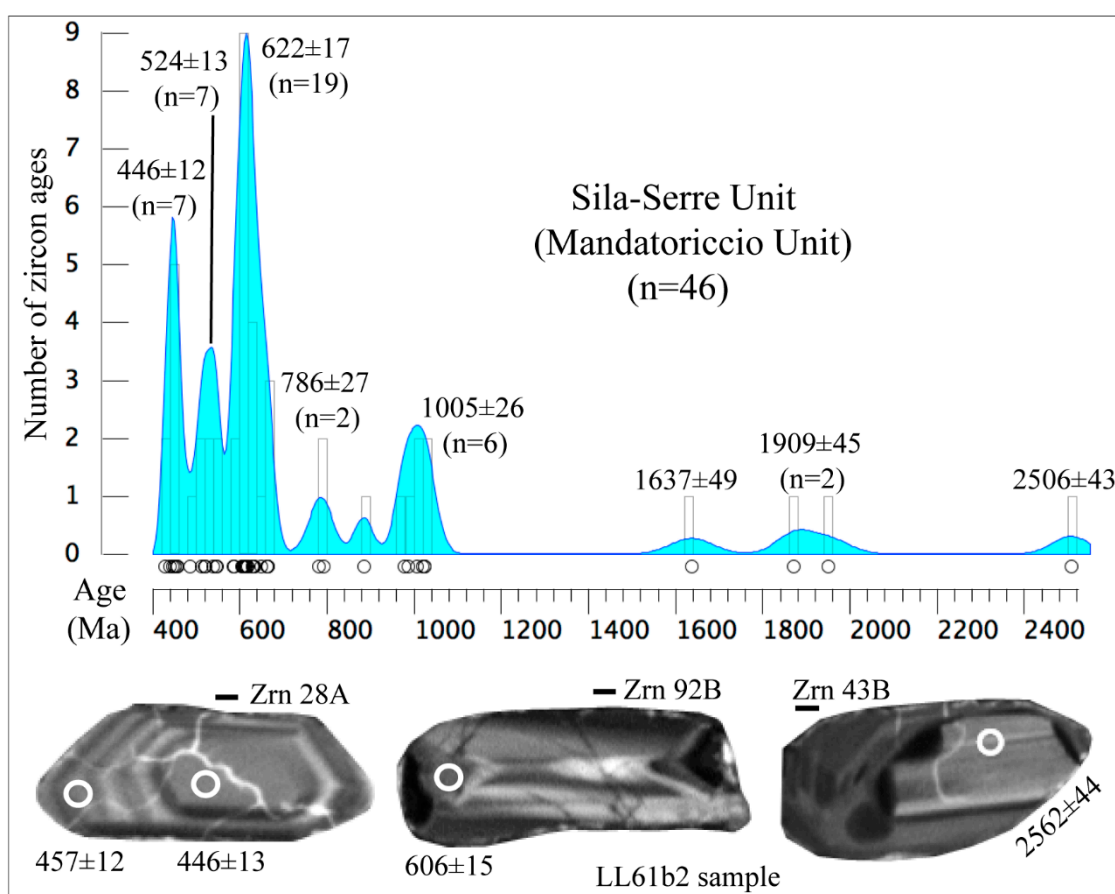
Figure 6. Histogram and probability density plot of zircon ages in paragneiss from the Mandatoriccio Unit (data from [71]). Spot ages in the selected zircons (CL images) reflect the main age clusters. Note the network of bright veins affecting Zrn28A. Zircons 28A, 92B, and 43B are modified after [70]. Symbols as in Figure 3.
