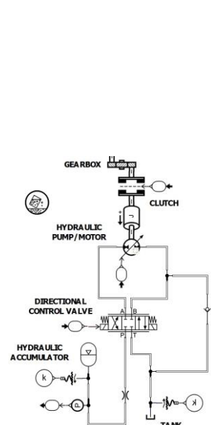
Fig. 4. Braking recovery system diagram.
