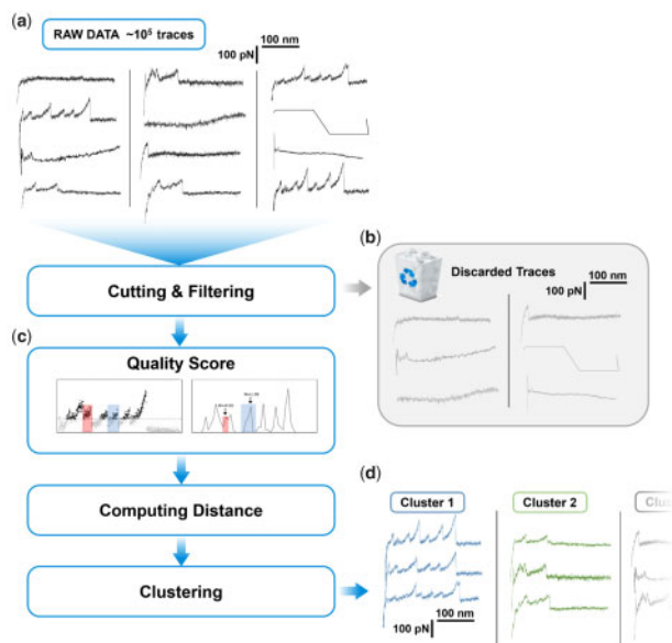
Fig. 1. Block scheme of the algorithm
