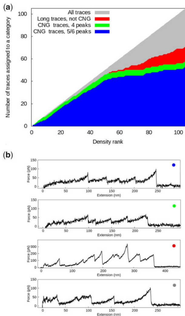
Fig. 2. Graphical representation of the CNG cluster content. (a) The cluster members are ranked by density in descending order. The blue area shows the manually selected CNG traces with five or six force peaks; the green area—manually selected CNG traces with 4 peaks; the red area—traces with contour length greater than 350 nm; the grey area corresponds to all traces assigned to the cluster. (b) Representative traces for the different groups in panel a. The painted dot in the top right corner indicates the group affiliation
