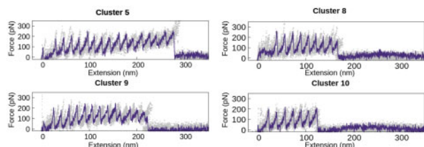
Fig. 3. Most representative cluster centres (blue lines) and closest 10 neighbours (grey points) of the dataset 'GB1'
