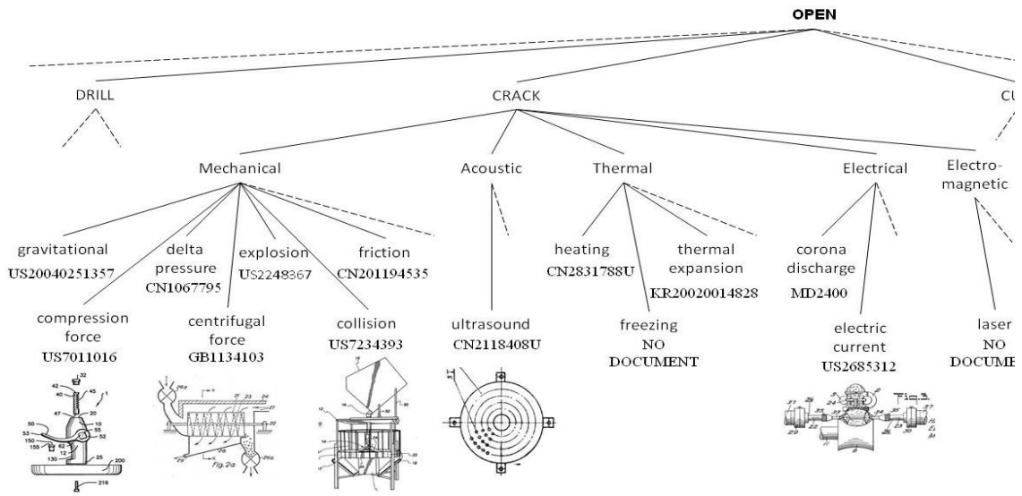
Figure 9. A partial representation of the SoA diagram of a nutcracker. Alternative systems of a traditional nutcracker are mapped, classified according to different effects (Ph).
