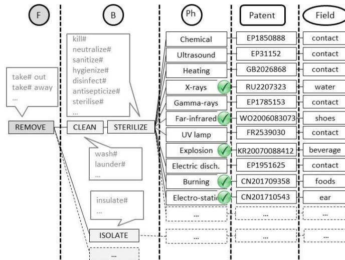
Figure 14. TT map: SoA and WSOs (ticked) found in different technical fields.
