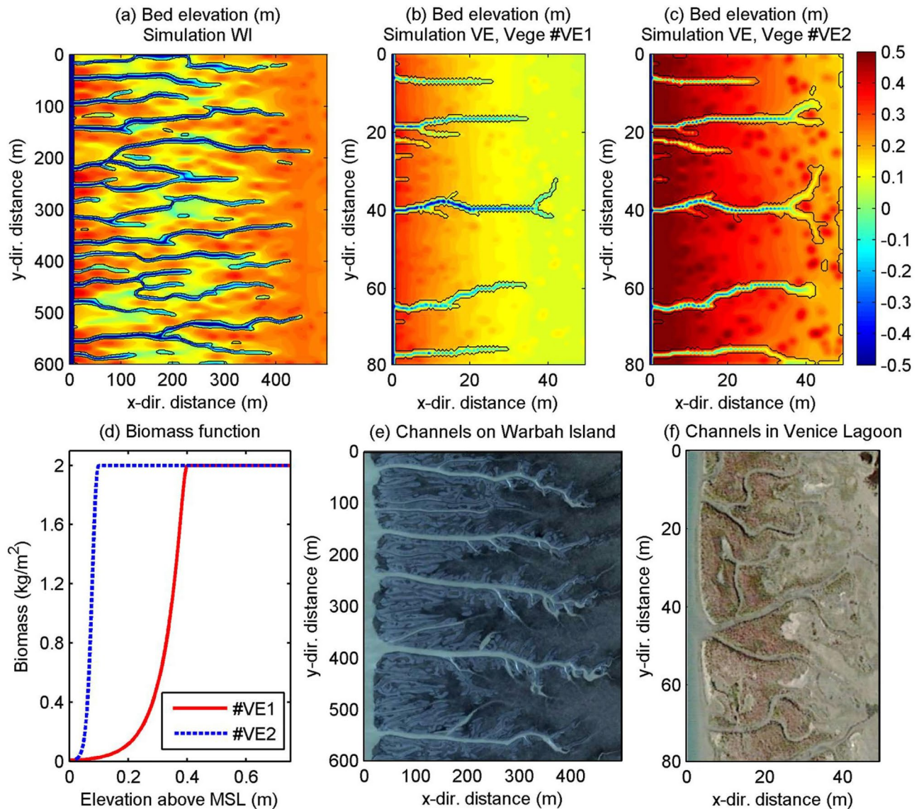
Figure 11. The bed topography (m above mean sea level [MSL]) obtained after 115 years in the simulations carried out for (a) Warbah Island and (b, c) a typical small salt marsh in the Venice lagoon. In this latter case, two different types of vegetation have been considered, Vege #VE1 and Vege #VE2, with biomass functions shown in plot (d). (e–f) Enlarged view of the actual channel morphologies observed in WI and VE.
