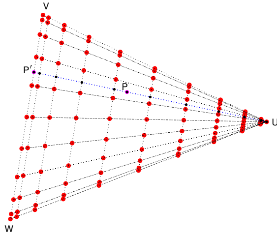
Figure 6: Chebyshev-Lobatto grid with m = 10 on the planar supporting triangle of a spherical triangle \mathcal{T} = \widehat{UVW} , cf. Fig. 1.
