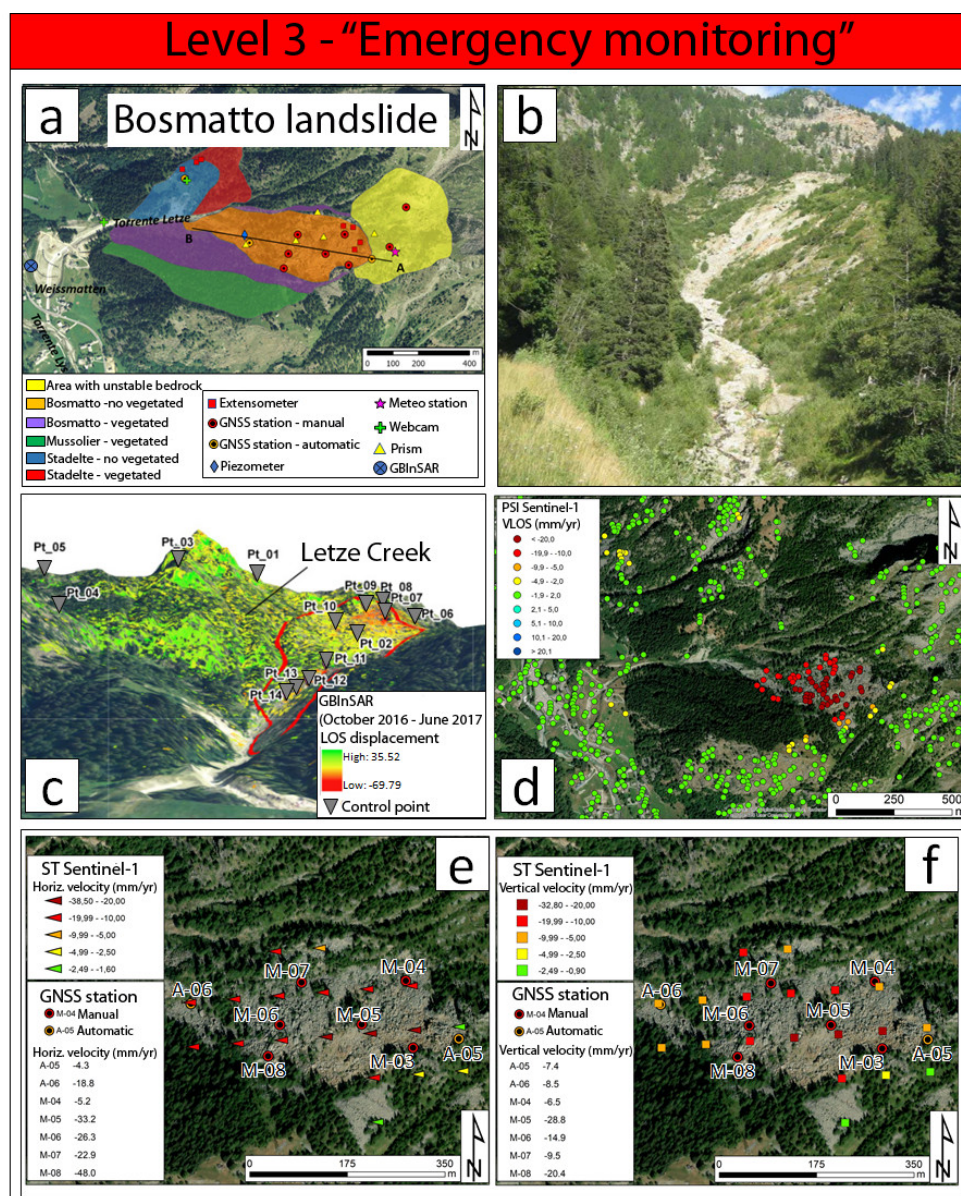
Figure 4. Level 3 - "Emergency monitoring": Bosmatto landslide: (a) geological map and location of instruments on the landslide; (b) photo of the Landslide from [41]; (c) ground-based interferometric radar system (GBInSAR) displacement data on the landslide; (d) Sentinel-1 PSI descending data on the landslide; (e) horizontal component of velocity of Synthetic Targets derived from PSI data and horizontal velocity recorded by global navigation satellite (GNSS) stations; (f) vertical component of velocity of Synthetic Targets derived from PSI data and vertical velocity recorded by GNSS stations.
