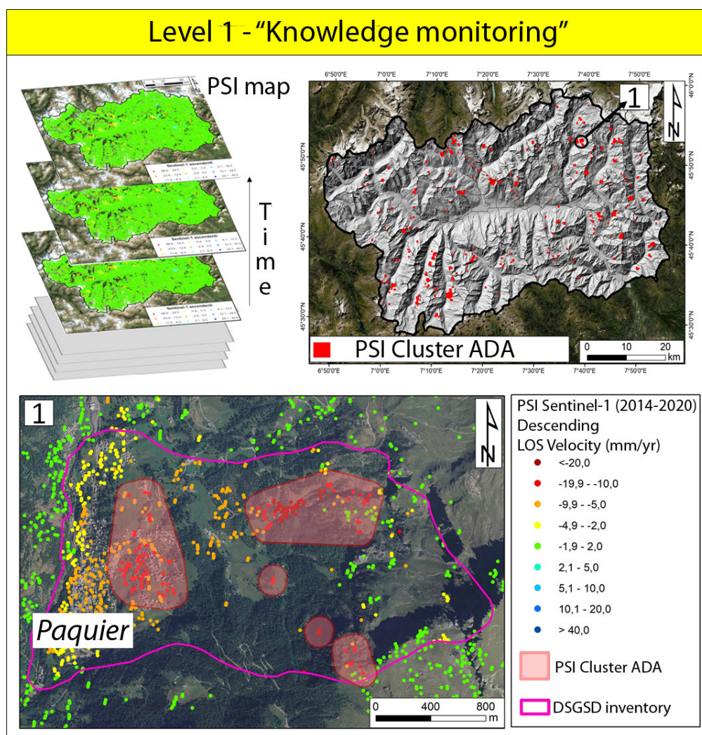
Figure 2. Level 1 – “Knowledge monitoring”: Concept of “PS mapping” activity ( top-left box ); distribution of Persistent Scatterer Interferometry (PSI) clusters named as Active Deformation Areas (ADA) for October 2014–August 2020 over the VAR ( top-right box ); example of PSI ADA clusters whose location is shown in the up-right box ( lower box ).
