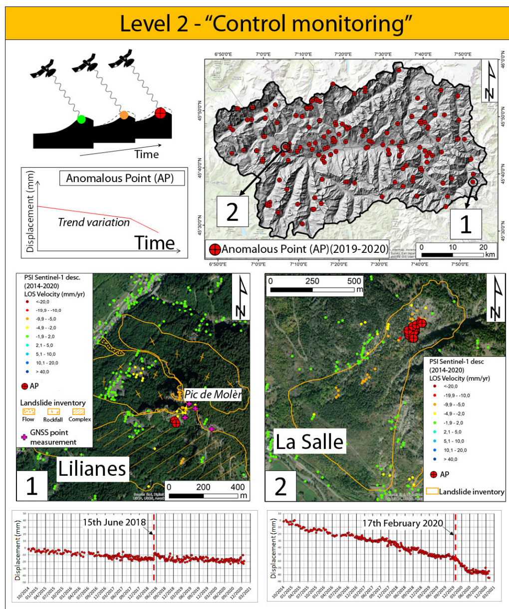
Figure 3. Level 2 – “Control monitoring”: Concept of “PS monitoring” (top-left box); Distribution of Anomalous Point targets (APs) in 2019–2020 within PS monitoring activity over the VAR (top-right box); two examples of APs, locations labeled (1) and (2), are shown in the top-right box (lower boxes).
