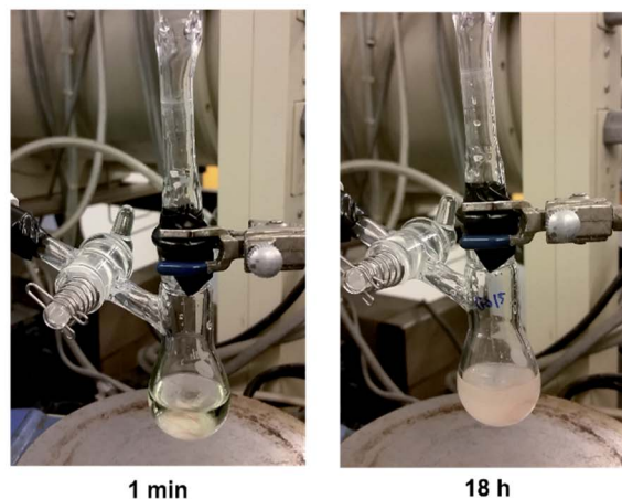
Fig. 4 Comproportionation of [\text{Cu}^{\text{I}}\text{Br}_2] = 2.5 \text{ mM} with [\text{TPMA}] = 5.25 \text{ mM} in the presence of [\text{QA}] = 10.0 \text{ mM} and 4 \text{ cm Cu}(0) wire ( d = 1 \text{ mm} , S = 1.27 \text{ cm}^2 ); in DMSO at 22^\circ \text{C} .
