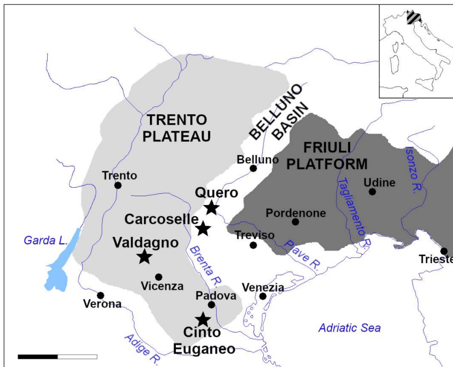
Fig. 1 - Sketch map of northeastern Italy with superimposed the main Cretaceous paleogeographic elements showing the position (black stars) of the fossiliferous localities examined in this study. Scale bar equals 50 km.
