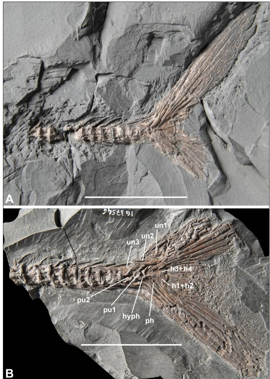
Fig. 22 - Pachyrhizodus sp.; Bomba Quarry (Cinto Euganeo). Posterior portion of the vertebral column, caudal skeleton and fin, A) MGCB IG37545, B) MGCB IG37546. Scale bars equal 50 mm.
