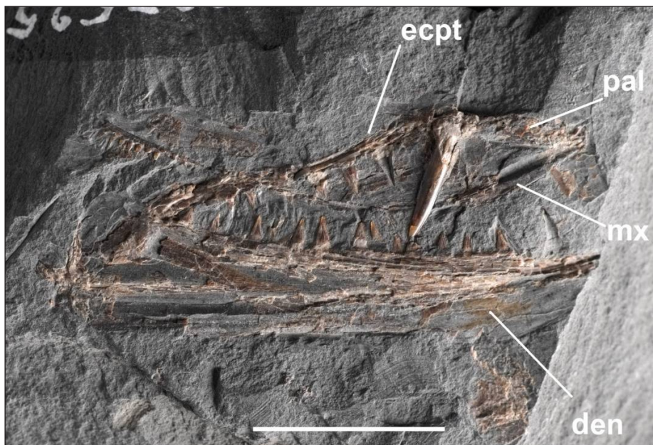
Fig. 36 - Rharbichthys ferax Arambourg, 1954; Bomba Quarry (Cinto Euganeo), MGCB IG37525. Scale bar equals 10 mm.
