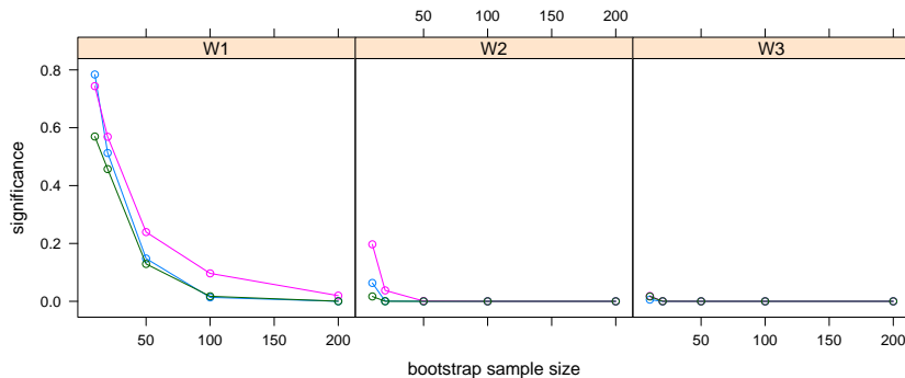
Figure 5.3: Monte Carlo significance values for the total variance (green), the generalized variance (blue) and the squared Frobenius matrix norm (violet) from Table 5.2.
