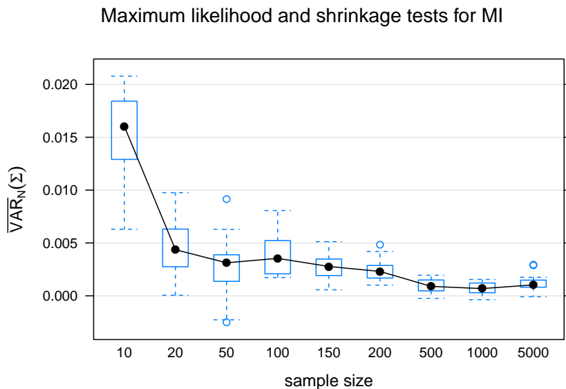
Figure 6.6: Difference in normalized total variance between the maximum likelihood and the shrinkage estimator for the mutual information. The black dot in each boxplot represents the median.
