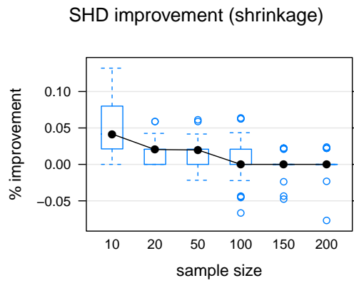
Figure 6.3: Improvements in Bayesian network structure learning when using the shrinkage estimator for the mutual information. The black dot in each boxplot represents the median.
