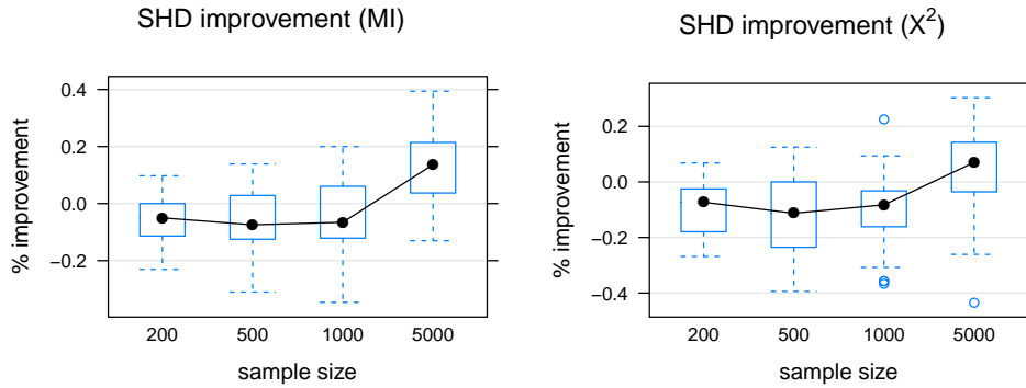
Figure 6.2: Differences in the Structural Hamming Distance when using permutation mutual information (on the left) and Pearson’s X^2 (on the right) tests. The black dot in each boxplot represents the median.
