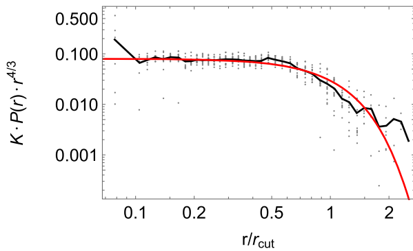
Fig. 5. Scaling collapse of the empirical diameter distributions of the 14 tropical forests. The gray dots are empirical rescaled points ( r/r_{cut} , K \cdot P(r) \cdot r^{4/3} ) for each forest, where r_{cut} is the best-fit value of the single adjustable parameter for each forest, K is the inverse of the normalization constant of the corresponding P(r) distribution and the exponent 4/3 = \alpha - 1 due to the choice of logarithmic binning). The black curve depicts the mean values of empirical points within each bin of the rescaled r/r_{cut} coordinates, while the red curve represents our prediction for the scaling collapse curve, e^{-x^{\alpha}} .
