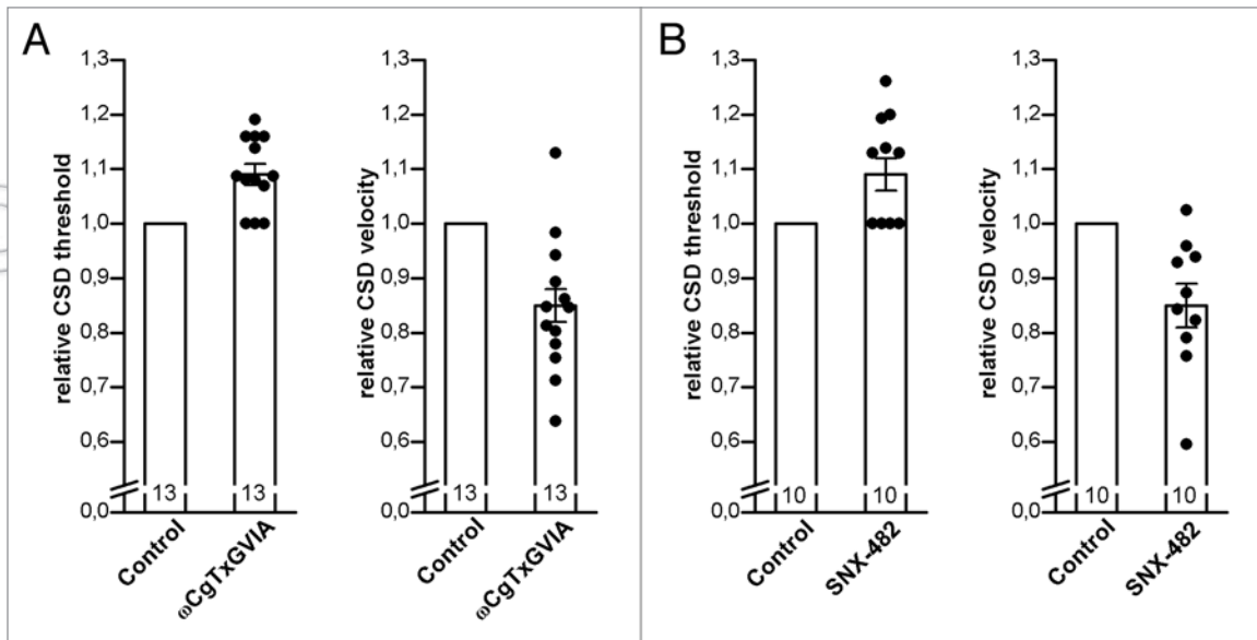
Figure 1. Relative values of CSD threshold and velocity before and after inhibition of N-type or R-type Ca 2+ channels. The threshold for CSD induction and the velocity of CSD propagation were measured before (control) and after application of saturating concentrations of \omega CgTxGVIA (A, n = 13) or SNX-482 (B, n = 10). The values obtained in the individual experiments in the presence of toxin relative to the corresponding control values are shown as dots and the average relative values as bar plots.
