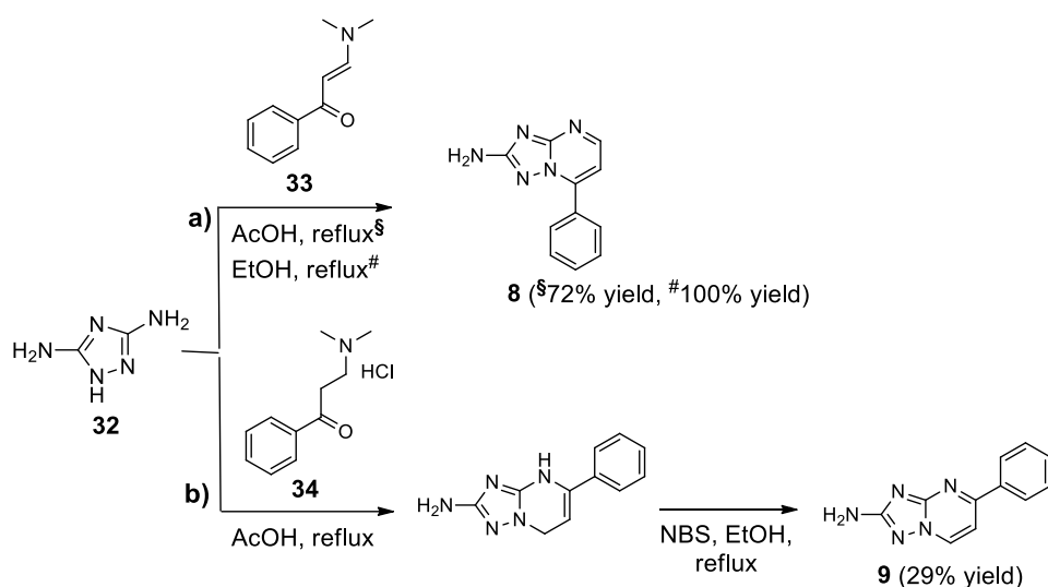
Scheme 1. Known procedures for the synthesis of 8 and 9 .
