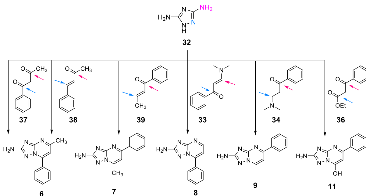
Figure 4. Plausible reactivity of 3,5-diamino-1,2,4-triazole ( 32 ) toward ambident electrophiles such as \beta -diketone ( 37 ), \alpha,\beta -enones ( 38 and 39 ), \beta -enaminone ( 33 ), \beta -amino ketone ( 34 ) and \beta -ketoester ( 36 ).
