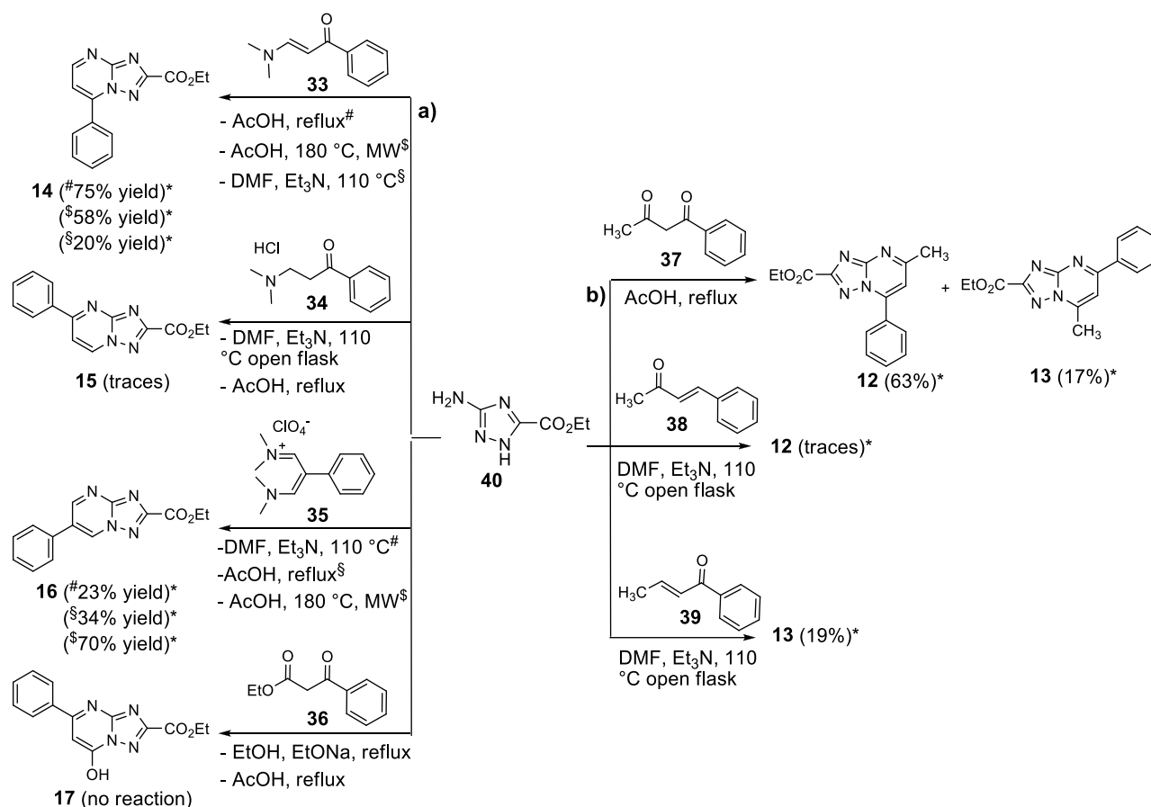
Scheme 2. Synthesis of 14-17 via reaction of 40 with 33-36 , respectively, and known procedures for the synthesis of 12 and 13 . *Isolated yields.
