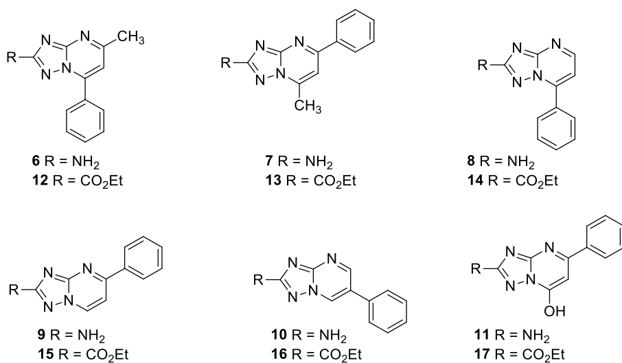
Figure 2. Structures of 1,2,4-triazolo[1,5- a ]pyrimidines variously functionalized at the C-5, C-6 and C-7 positions useful for the synthesis of IV RdRP PA-PB1 inhibitors.
